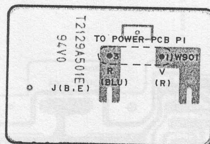
POWER TRANS PCB (2) T2I29A501E
