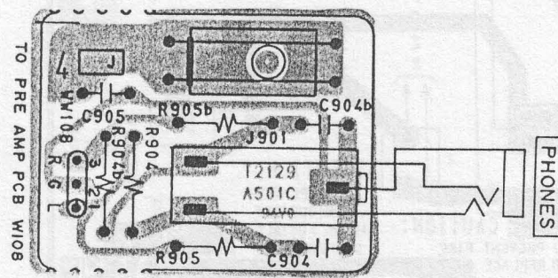
PHONE PCB T2I29A501C
