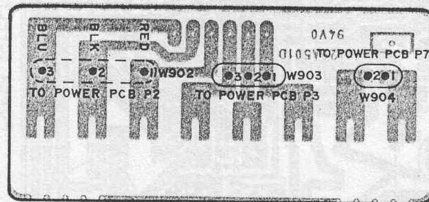
POWER TRANS PCB (1) T2I29A501D
