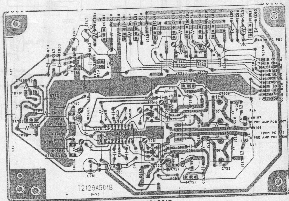
OSC PCB T2129A501B
