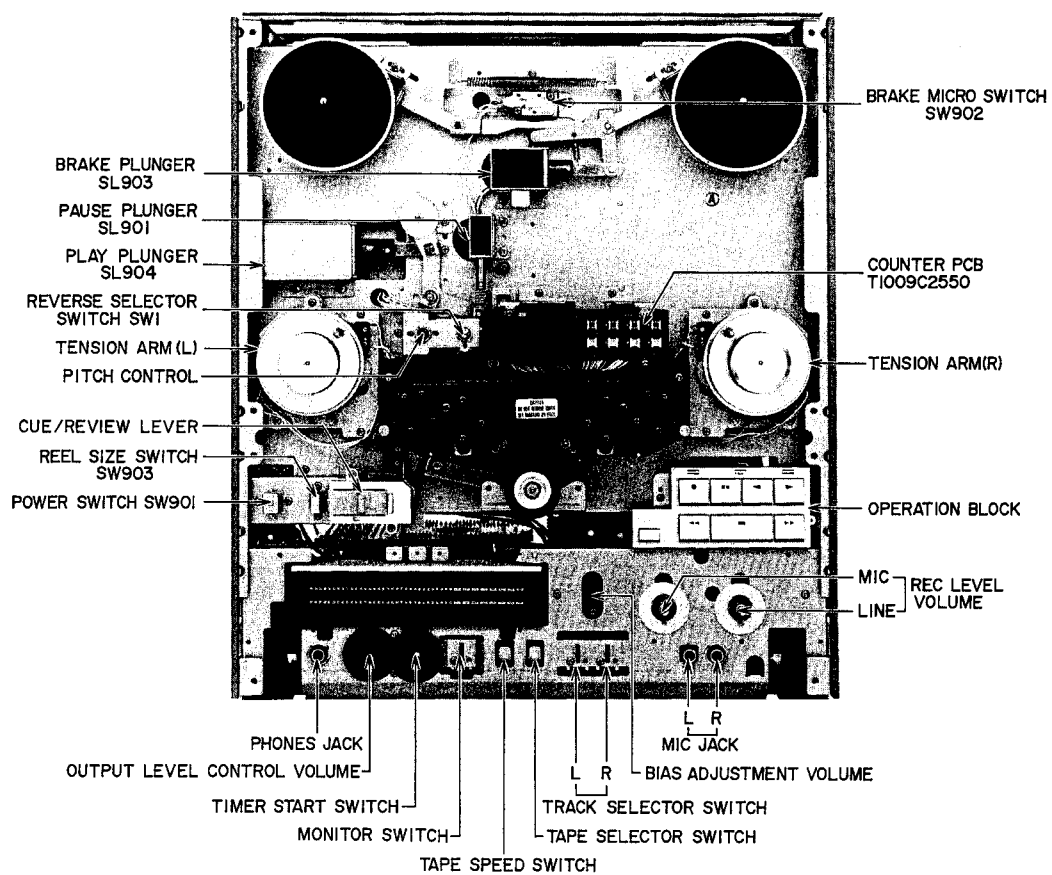
Fig. 2 Front View
