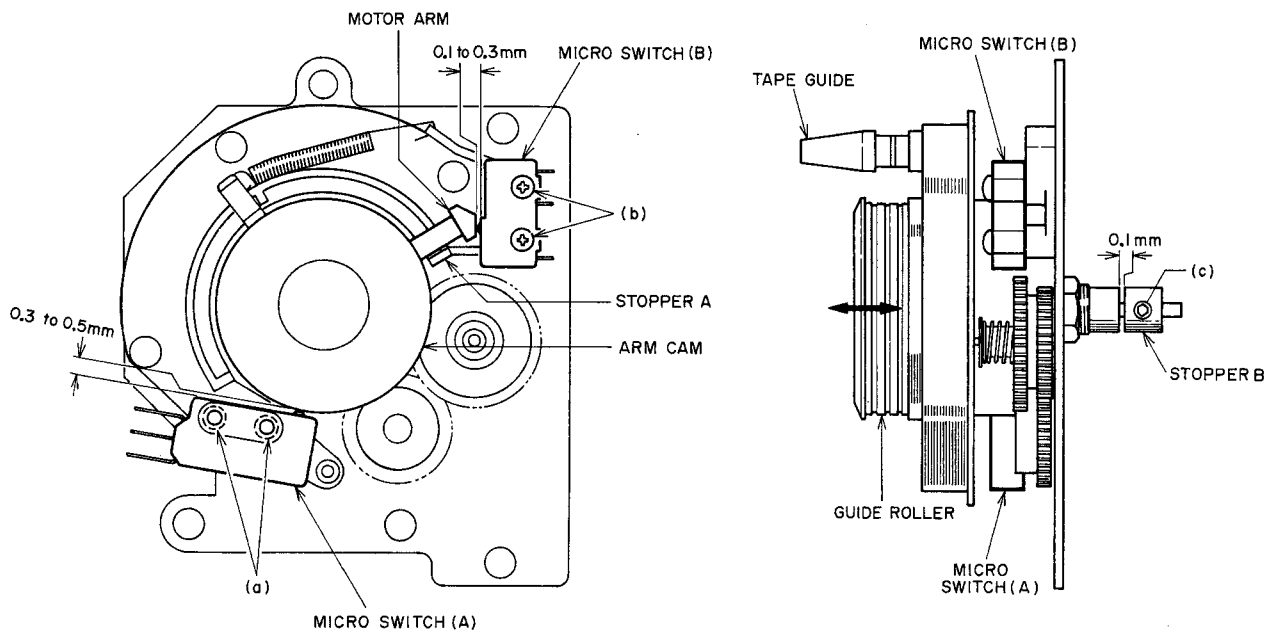
Fig. 33 Roller Block
