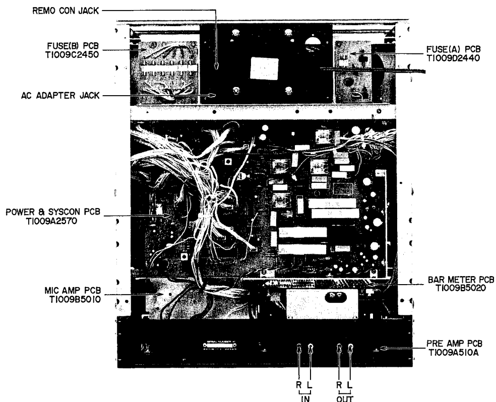
Fig. 3 Rear View
