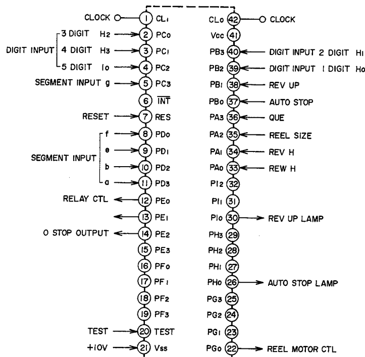
② IC2 Terminal Description
