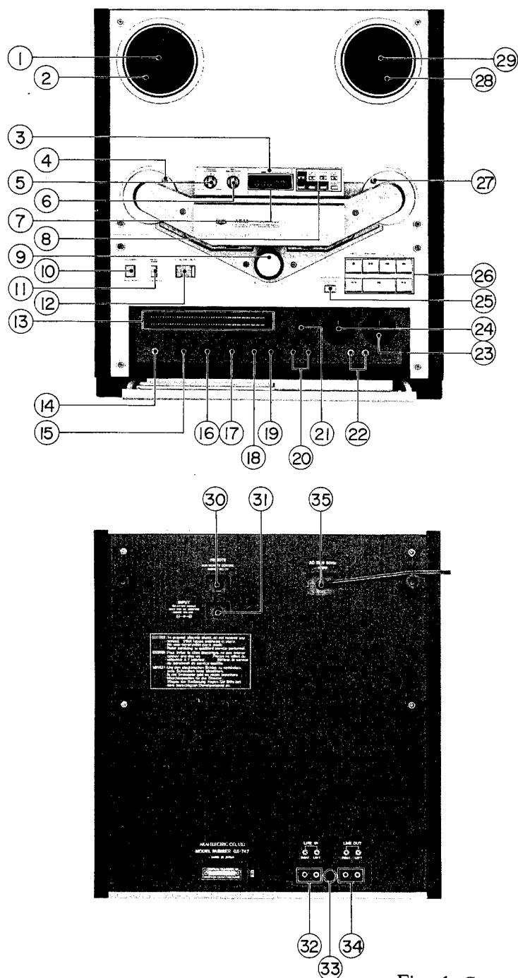
Fig. 1 Controls
