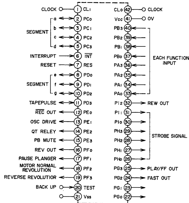
① IC1 Terminal Description
