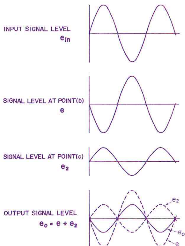
Fig. 42 Levels and Phases of Various Points at Individual Frequencies
