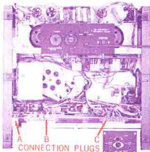
CONNECTION PLUGS
