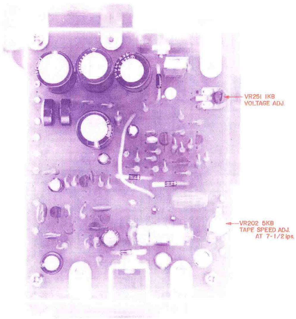
Fig. 35 SERVO CONTROL AMP. & POWER SUPPLY P.C. BOARD (FACE SIDE)
