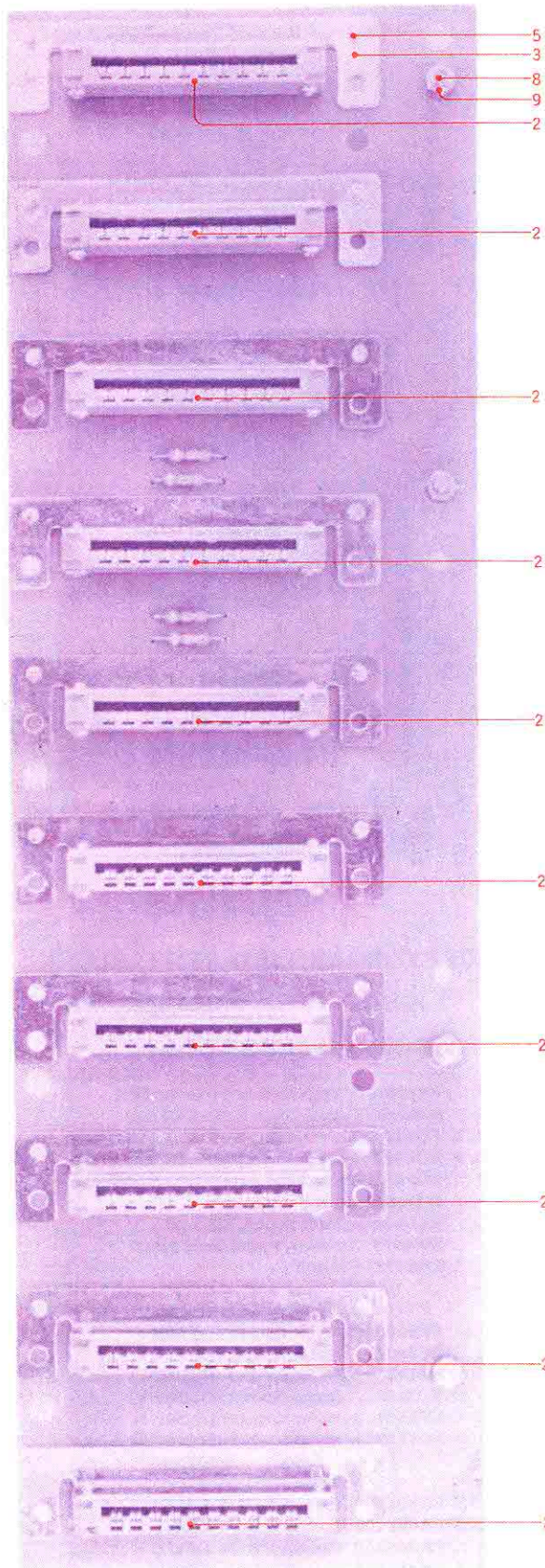
FIG. 15 PHOTO OF PRE-AMP. CHASSIS P.C. BOARD (KD-A5216)
