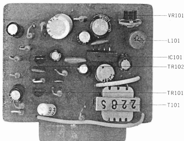
FIG. 8 PHOTO OF P.B. AMP. P.C. BOARD (KD-A5010)
