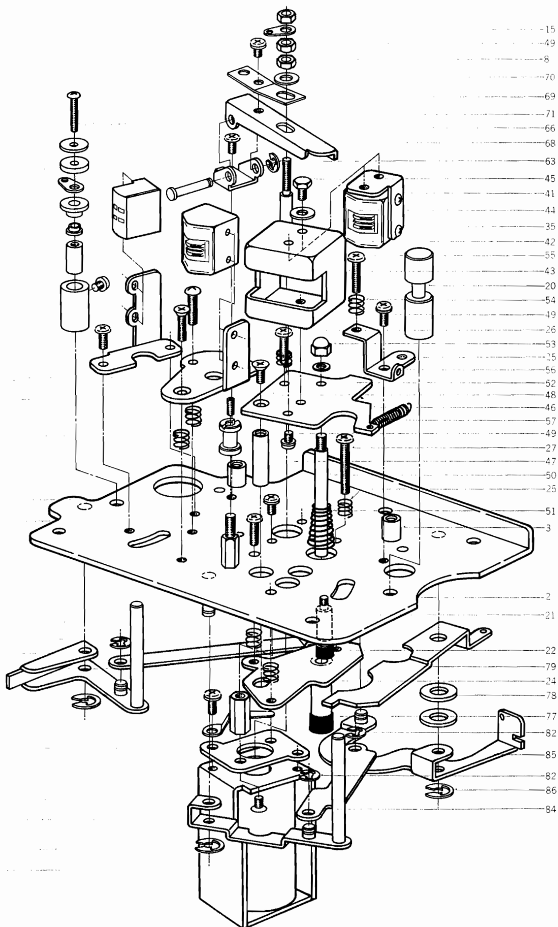
FIG. 1 ILLUSTRATION OF KG HEAD BLOCK
