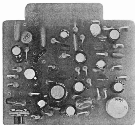
Fig. 22 RECORDING AMP. P.C. BOARD KD-A5011 (Face Side)
