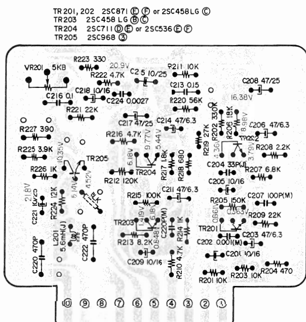
Fig. 21 RECORDING AMP. P.C. BOARD KD-A5011 (Reverse Side)
