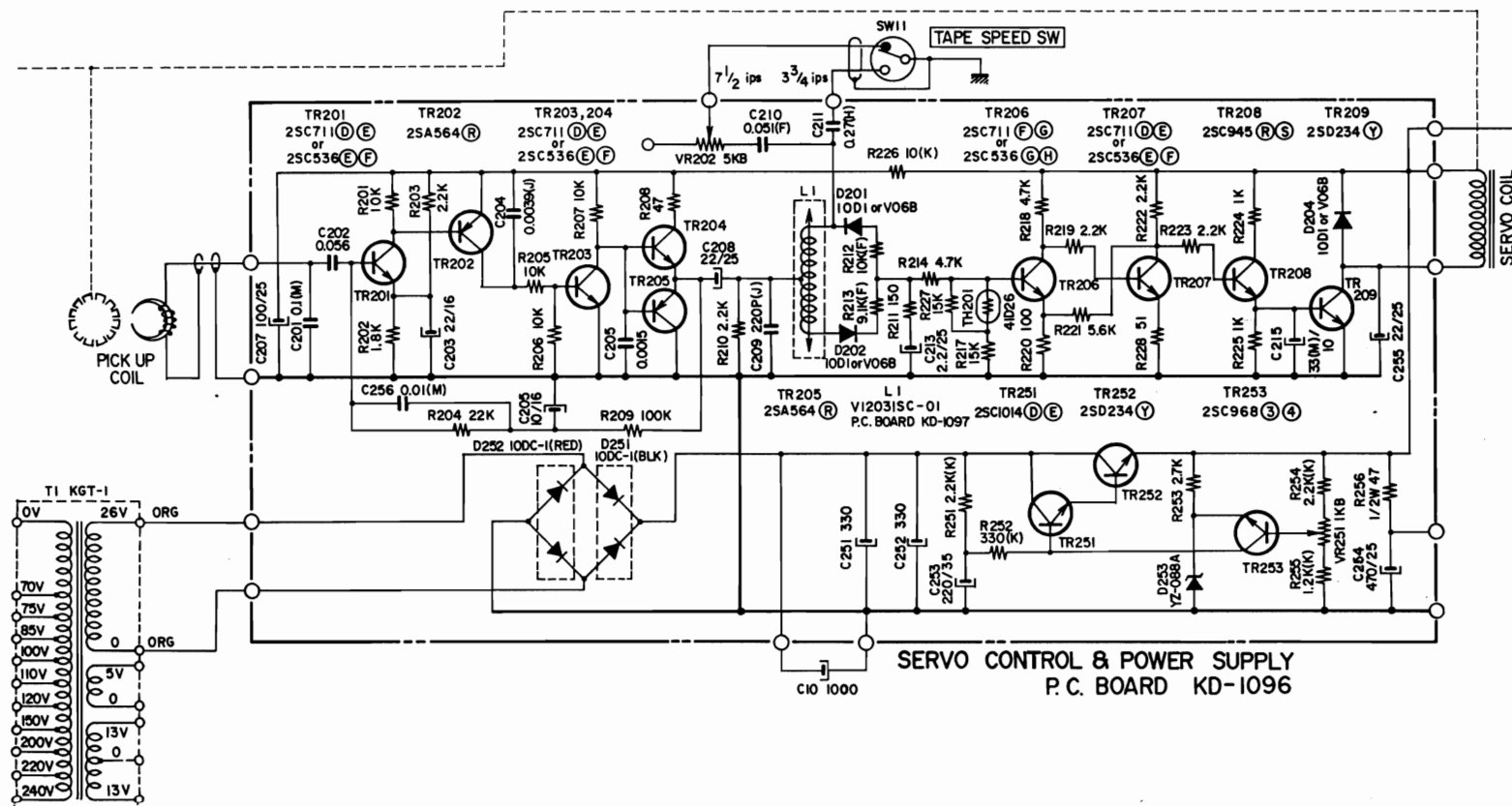
SCHEMATIC-2
