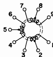
OSCILLATOR COIL
