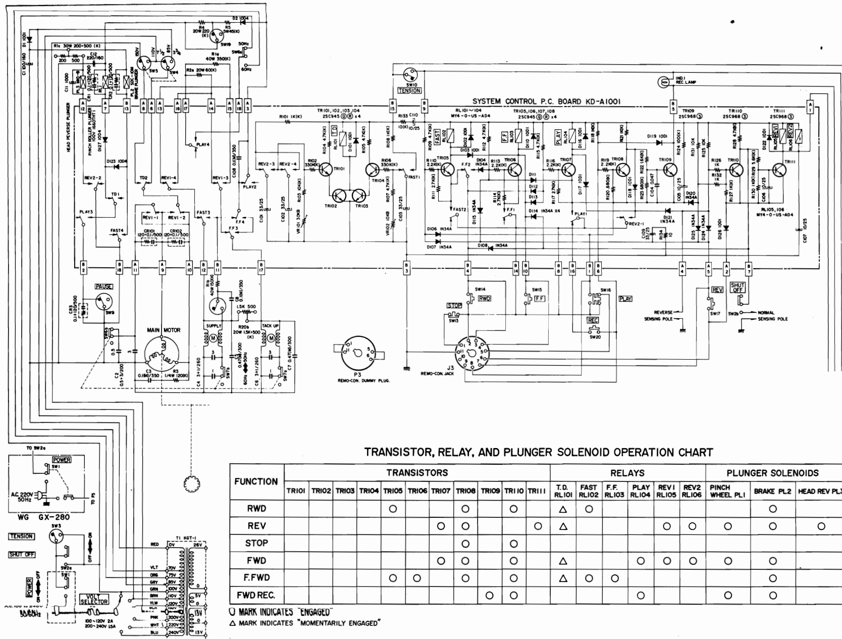
SYSTEM CONTROL SCHEMATIC DIAGRAM
