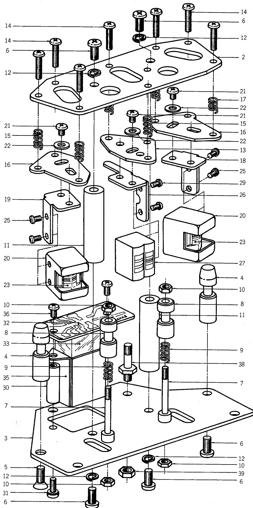
FIG. 1 HEAD BLOCK
