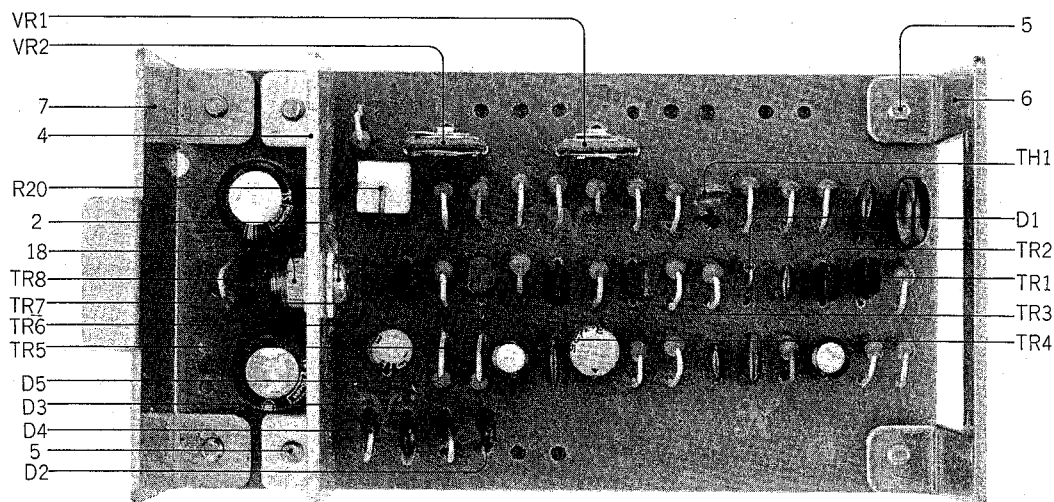
FIG. 12 SERVO P.C. BOARD (MY-2036) BLOCK
