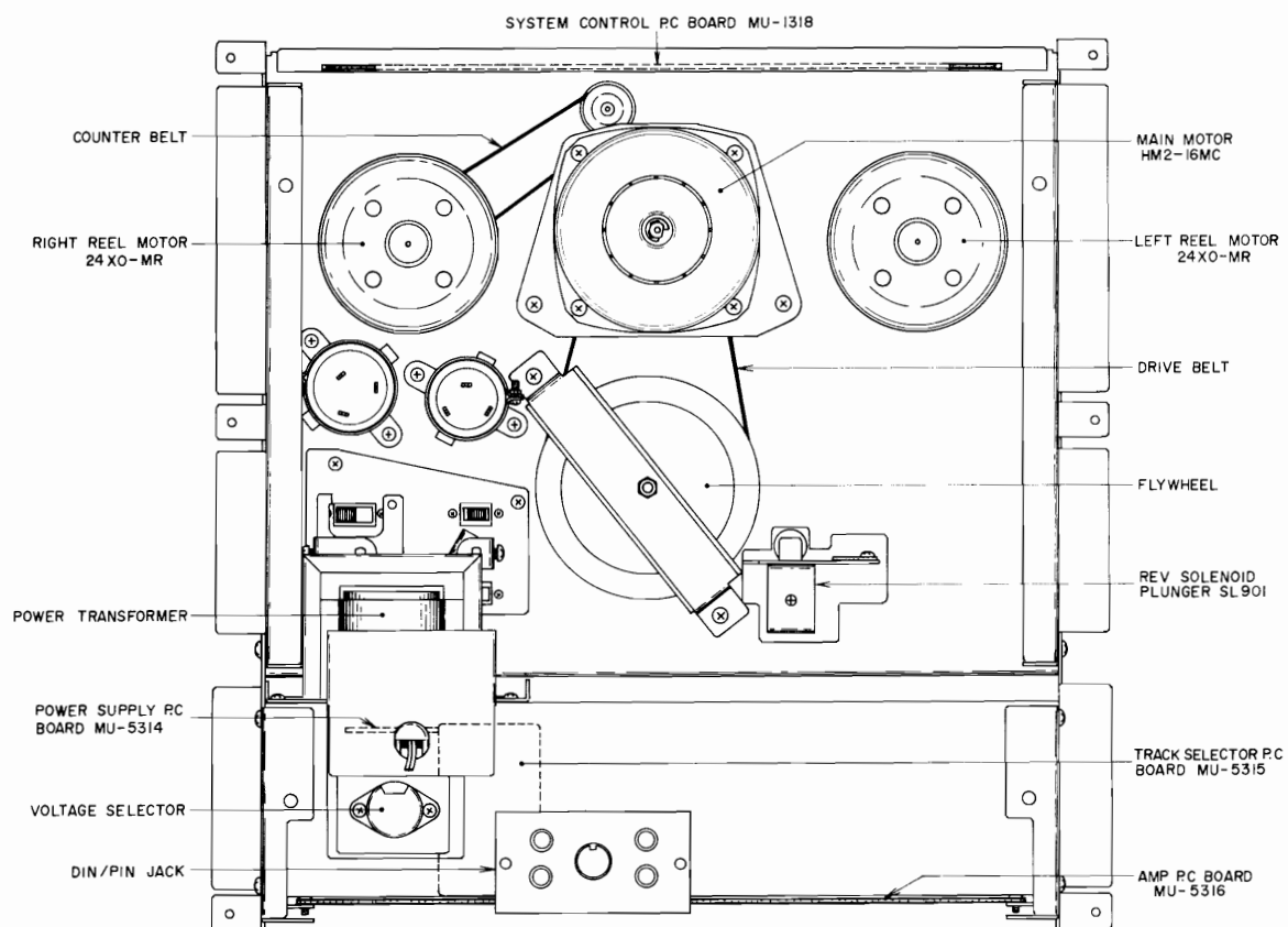
Fig. 3 Rear View
