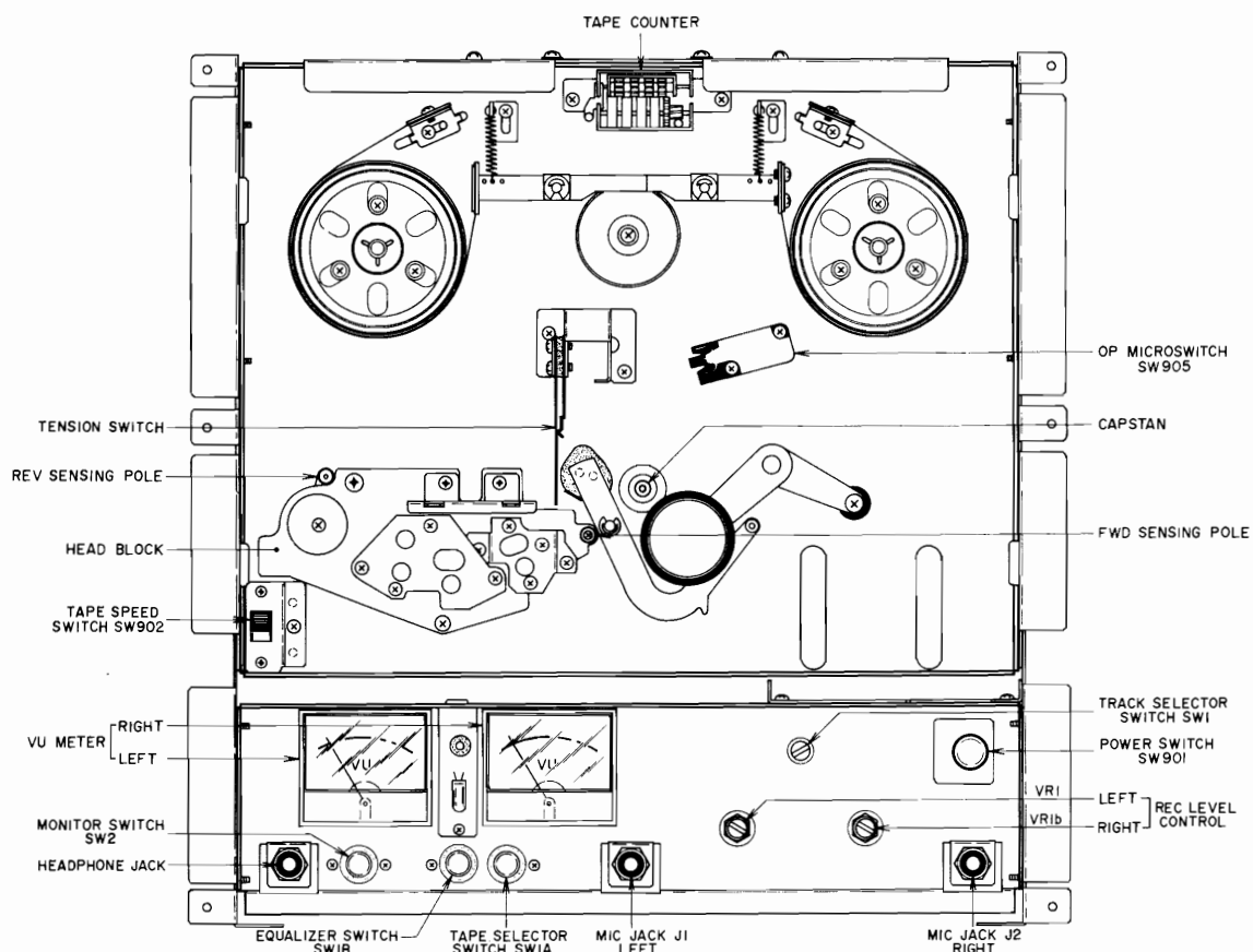
Fig. 2 Front View
