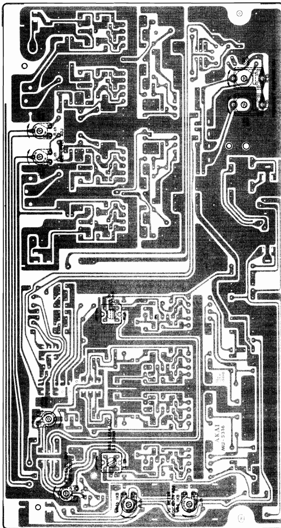
Fig. 10 Amp P.C Board MU-5316
