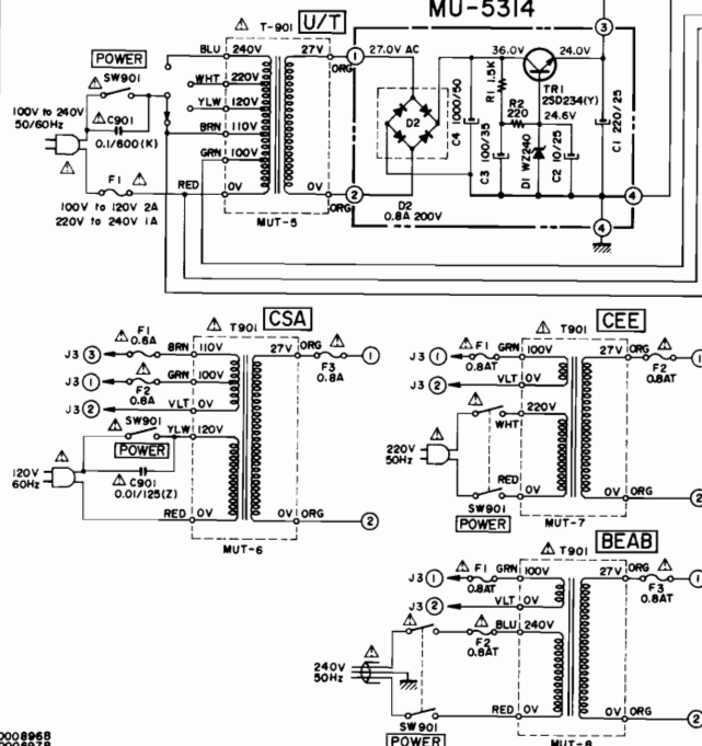
POWER SUPPLY PC BOARD MU-5314
