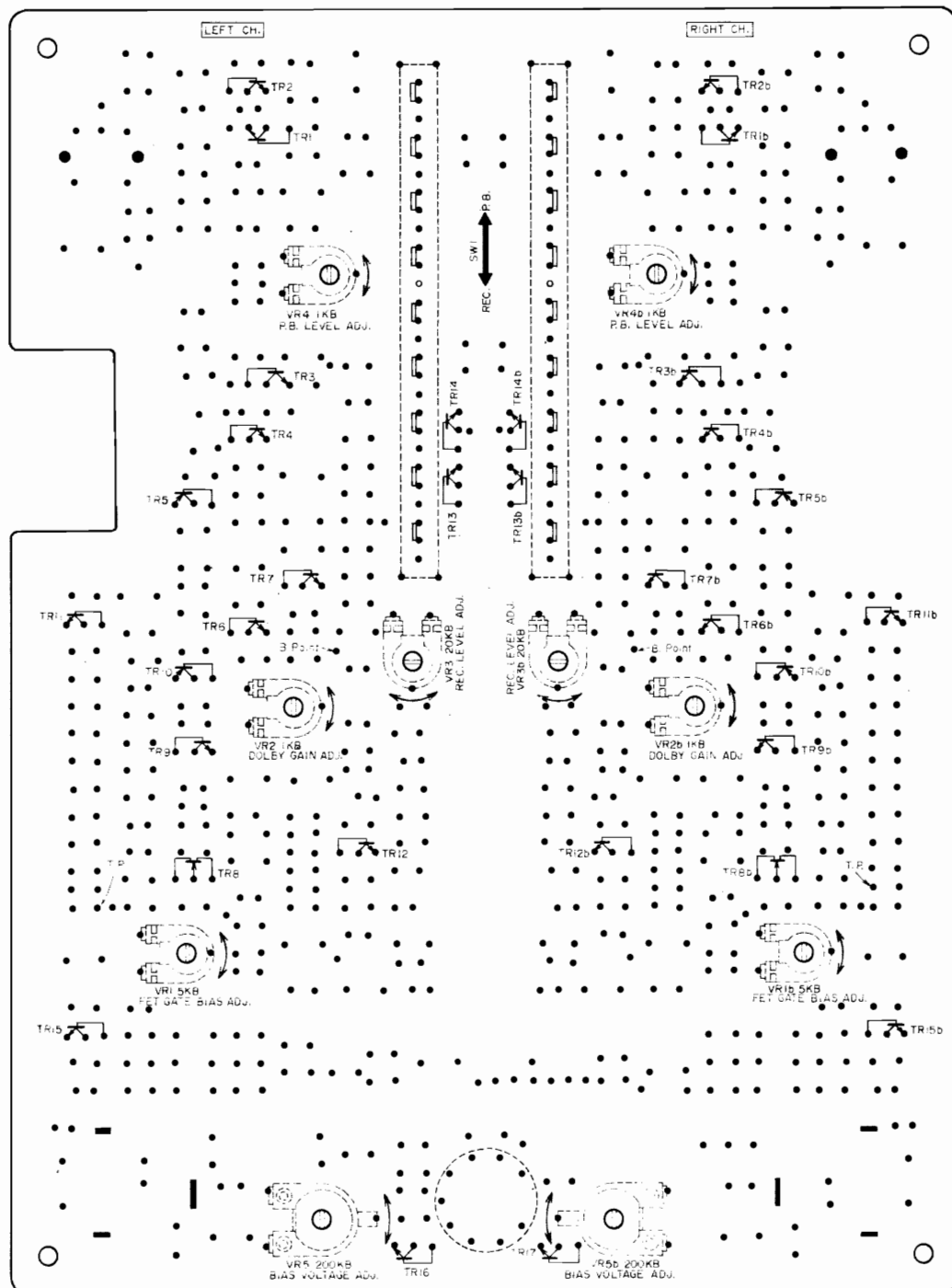
Adjustment points of Pre-Amp P.C. Board (CW-5214 2ED)
