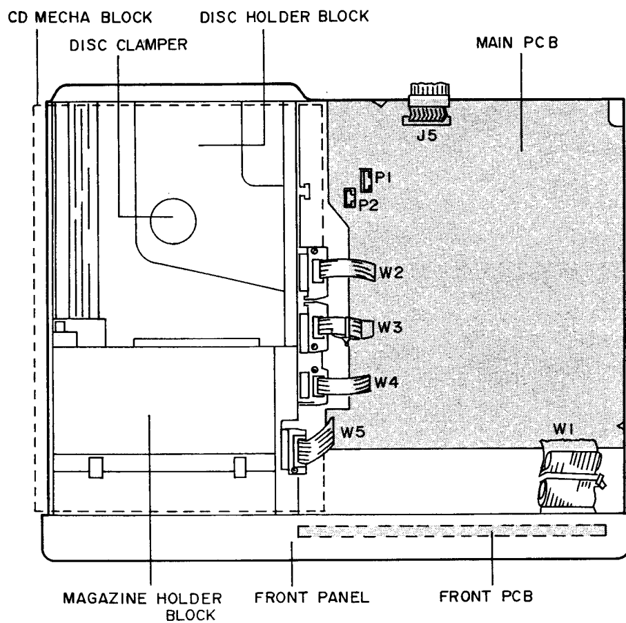
Fig.2-1 Top view
