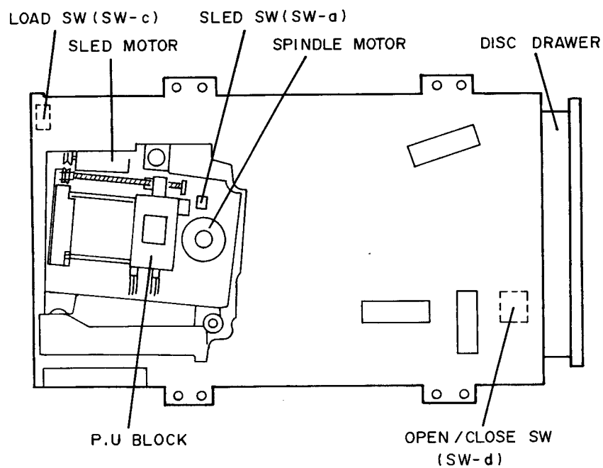
Fig.2-3 Bottom view
