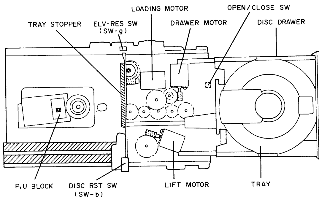
Fig.2-2 Top view
