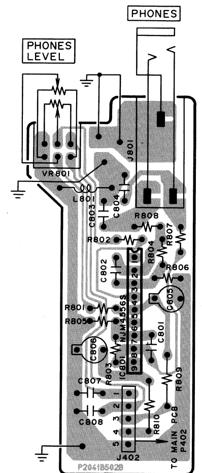
HEAD PHONE PCB P2041B502B
