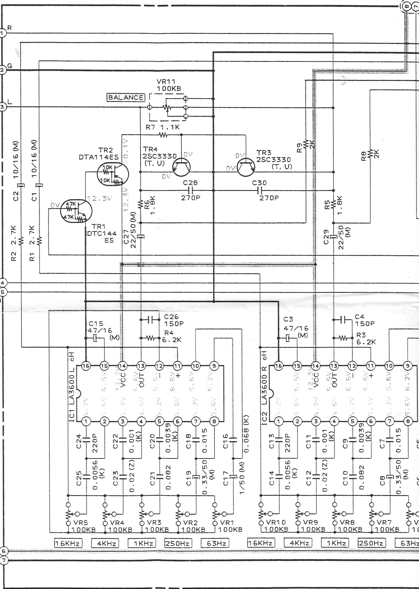
GEQ PCB C1028A503A
