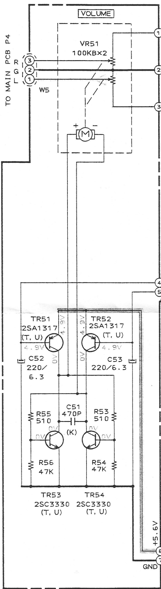
MAIN VR PCB C1028A503B
