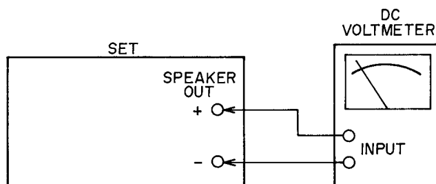
Fig. 11 Instrument Connections for Center Off-set Voltage Adjustment
