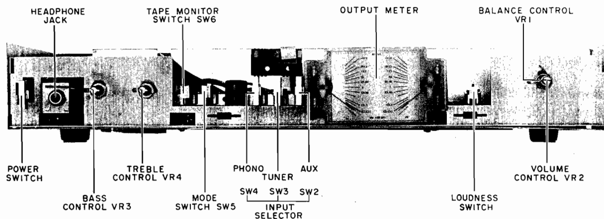
Fig. 3 Front View
