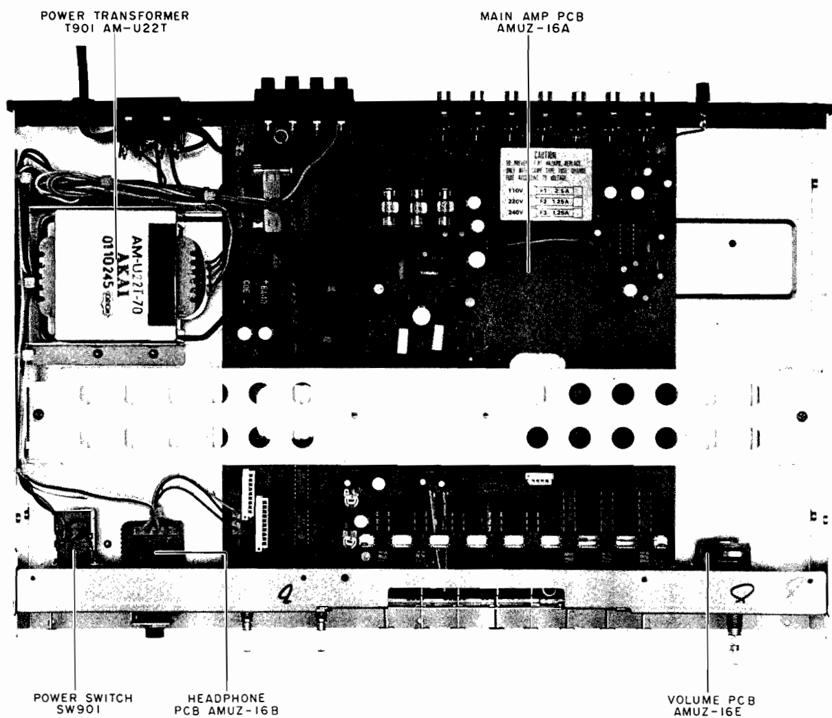
Fig. 6 Top View
