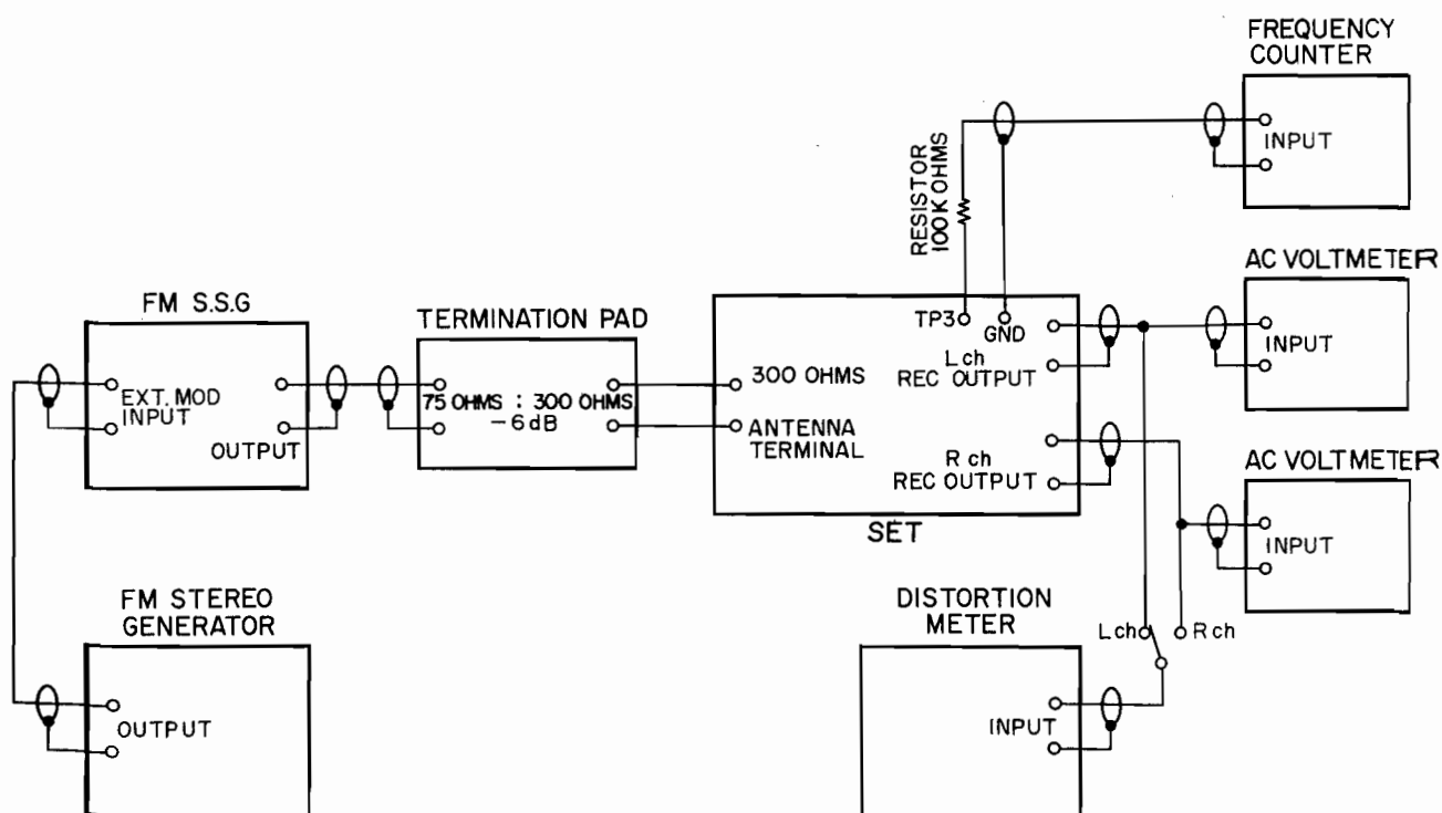
Fig. 11 Instrument Connections
