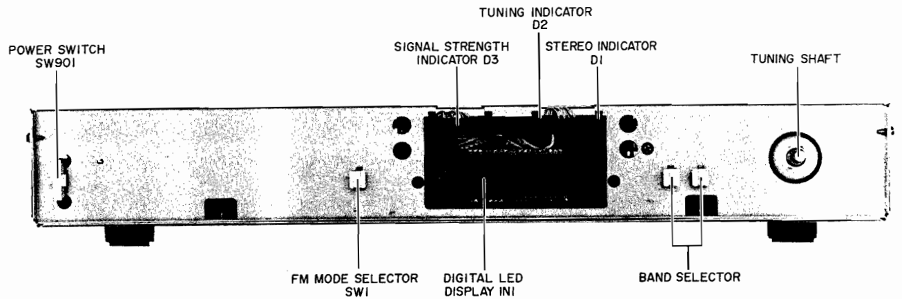
Fig. 5 Front View
