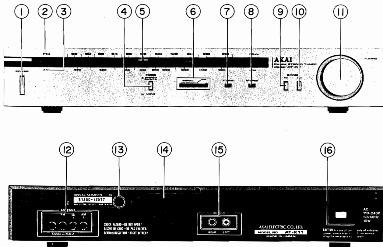
Fig. 1 Controls (AT-K11/L)
