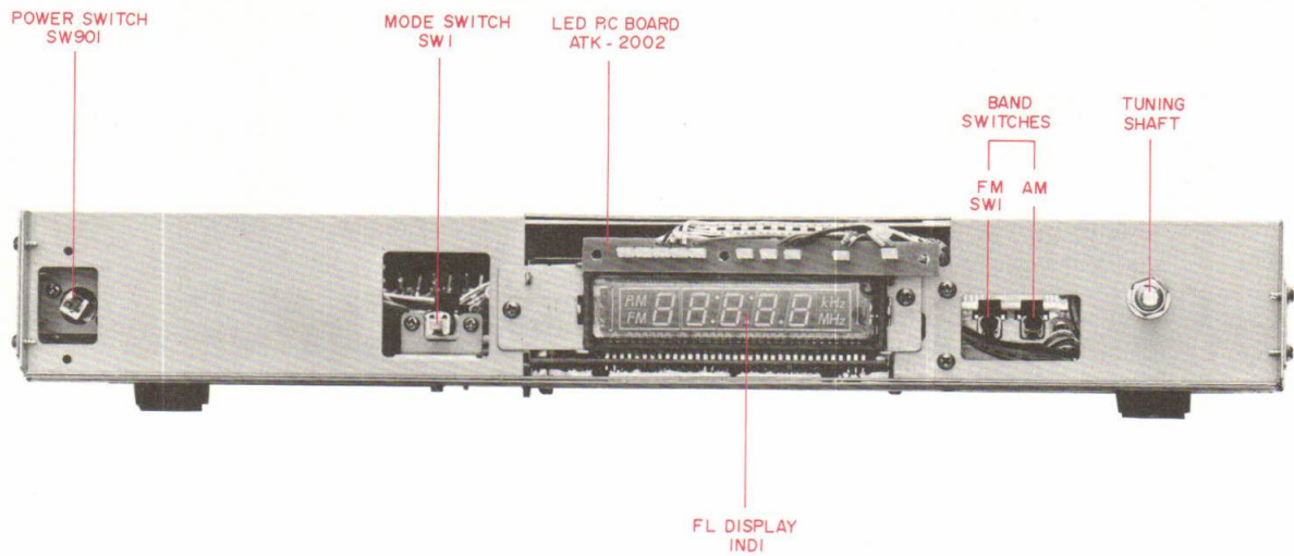
Fig. 2 Front View
