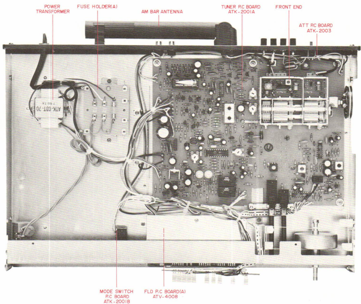
Fig. 3 Top View
