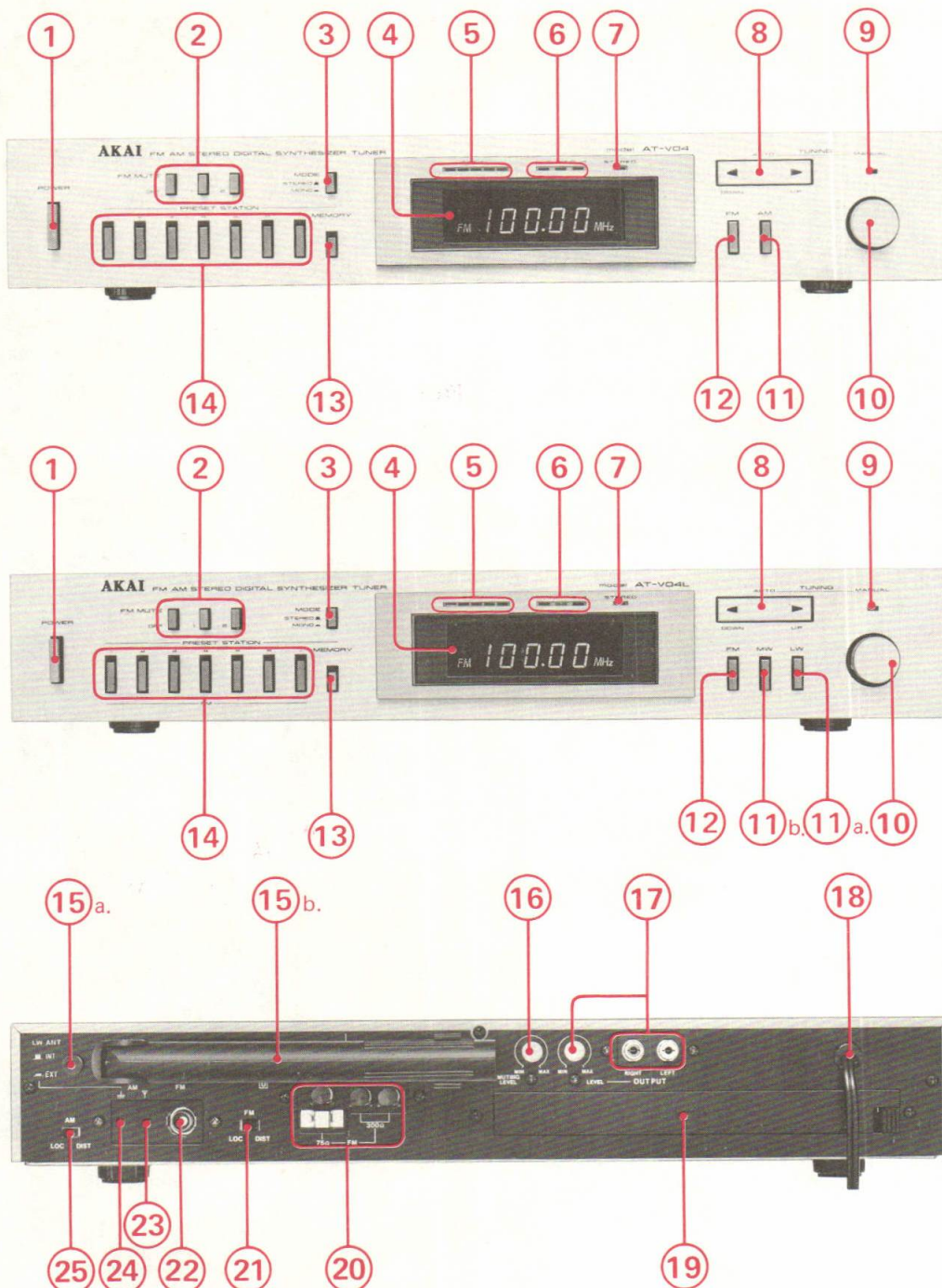
Fig. 1 Controls
