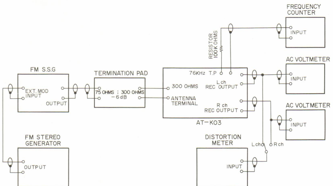
Fig. 7 Instrument Connections
