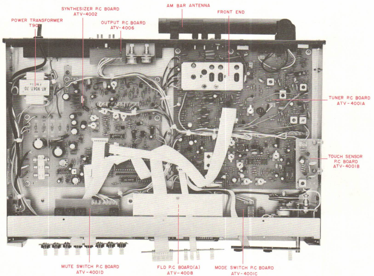
Fig. 3 Top View
