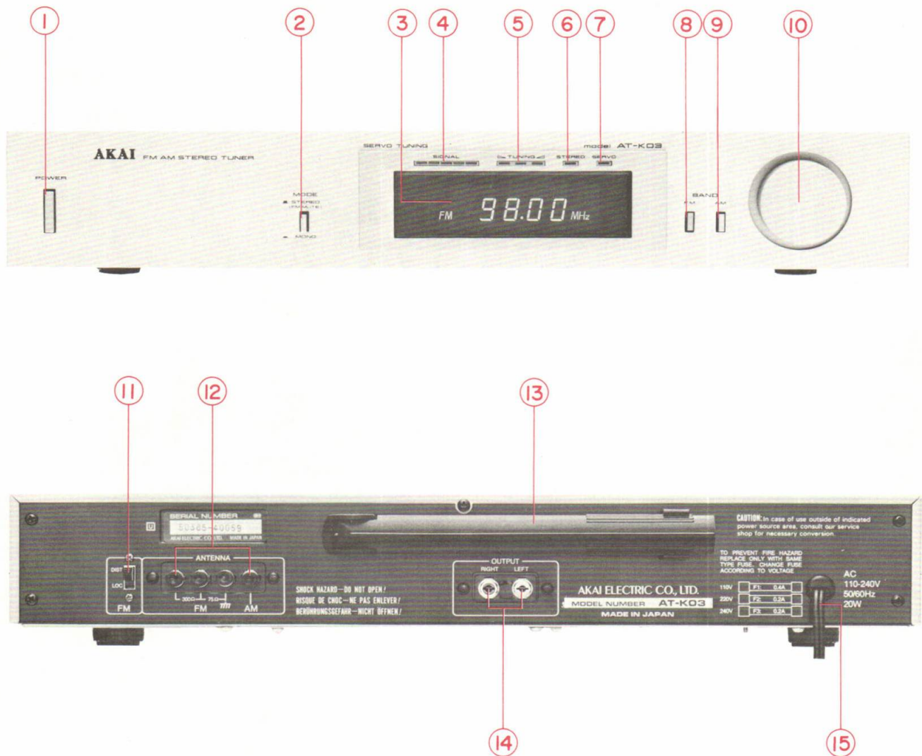
Fig. 1 Controls
