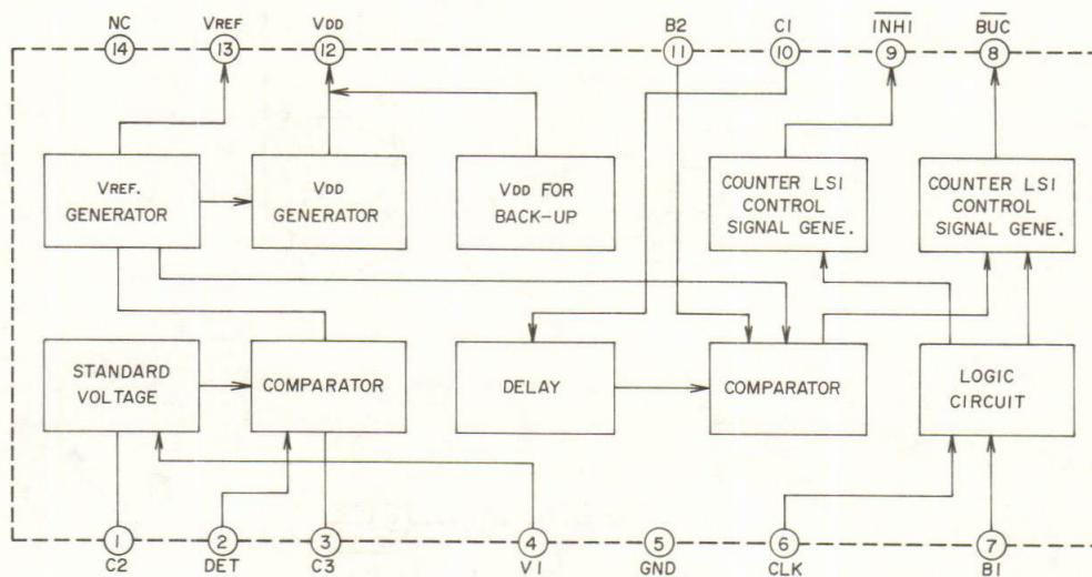
LOGIC CHART
