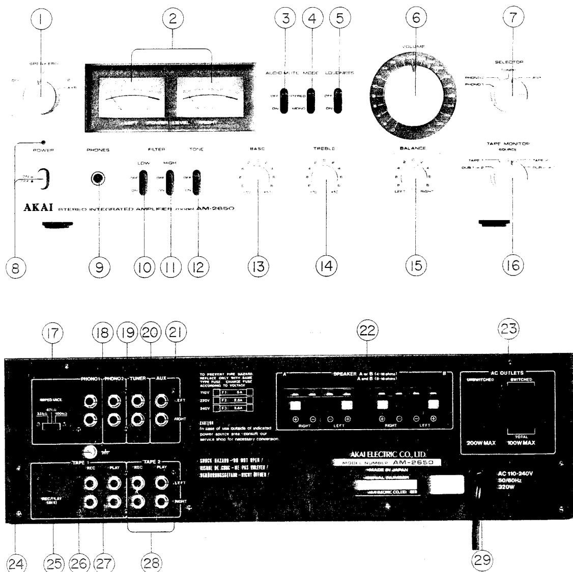
Fig. 2 Controls AM-2650
