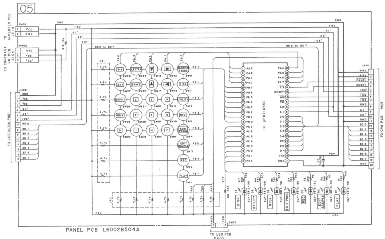
S900 PANEL SCHEMATIC DIAGRAM NO.6-4 860917A
