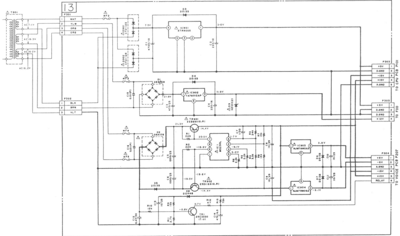
S900 POWER SUPPLY SCHEMATIC DIAGRAM NO.6-3 860915A
