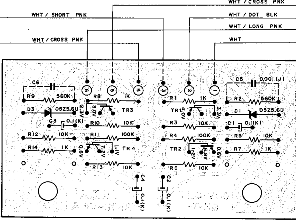
SIZE DETECTOR P.C BOARD APQ-8048
