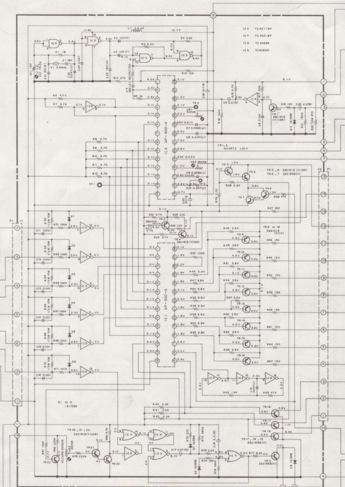
SYNTHESIZER P.C. BOARD APQ-7049
