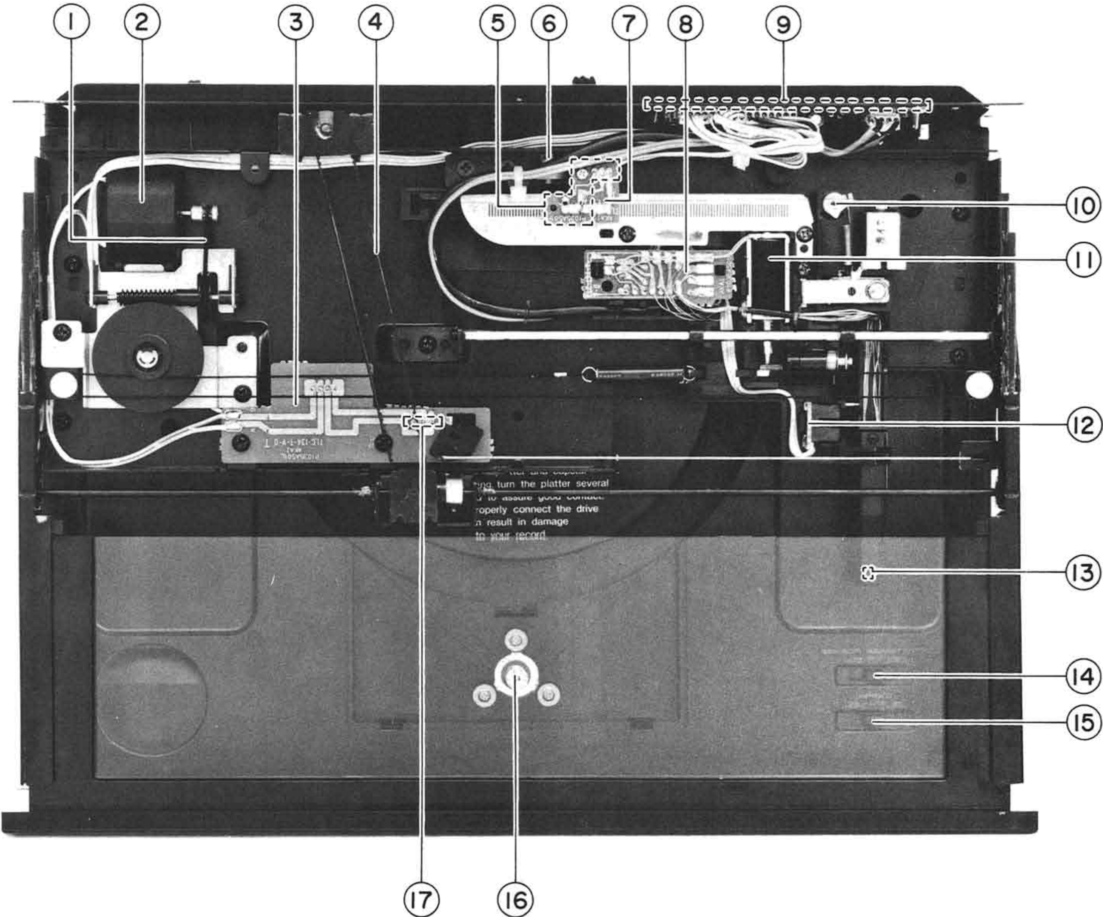
Fig. 4-1 Top View
