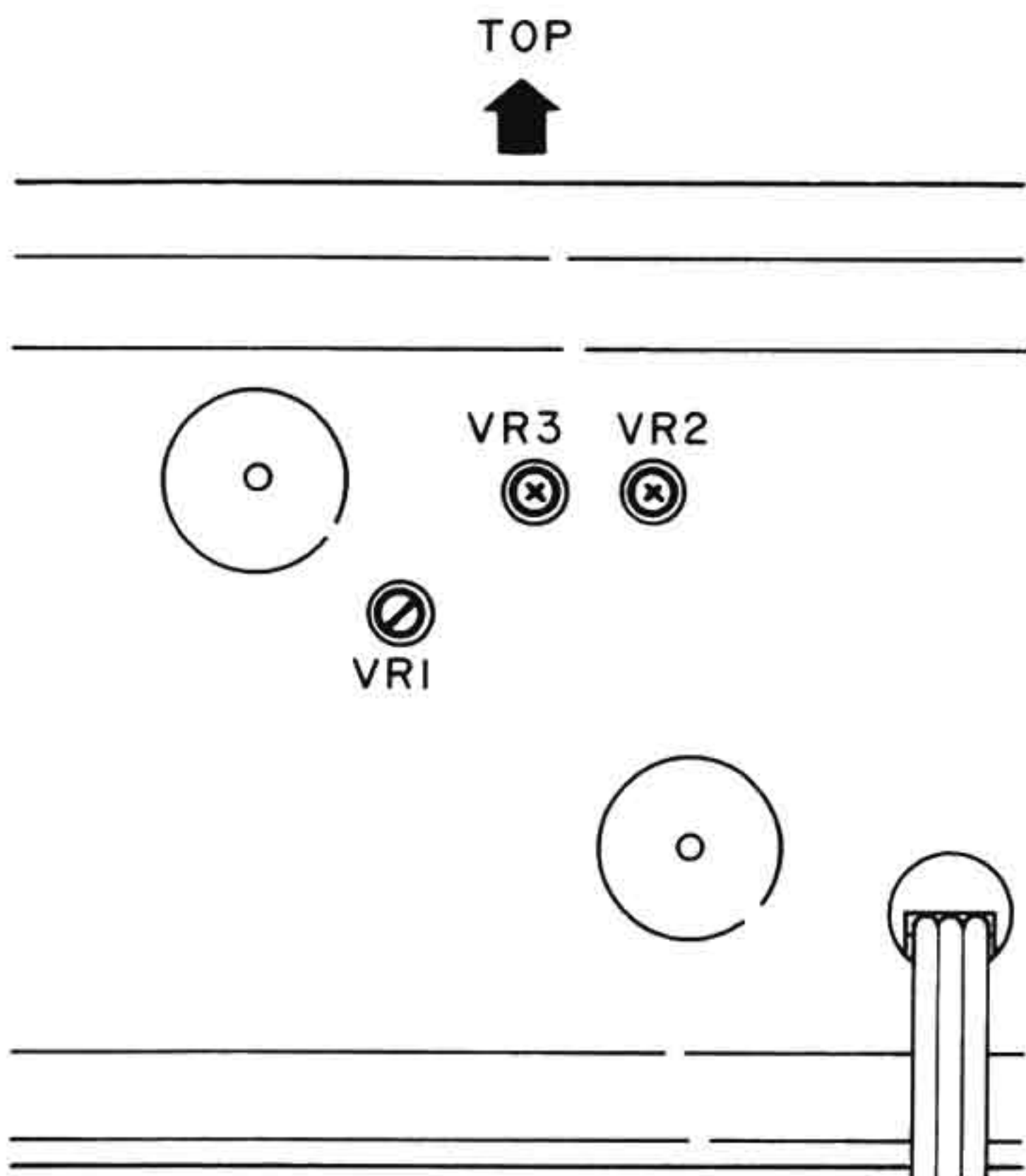
Fig. 6-2 Audio PCB ADJ Points (Rear View)
