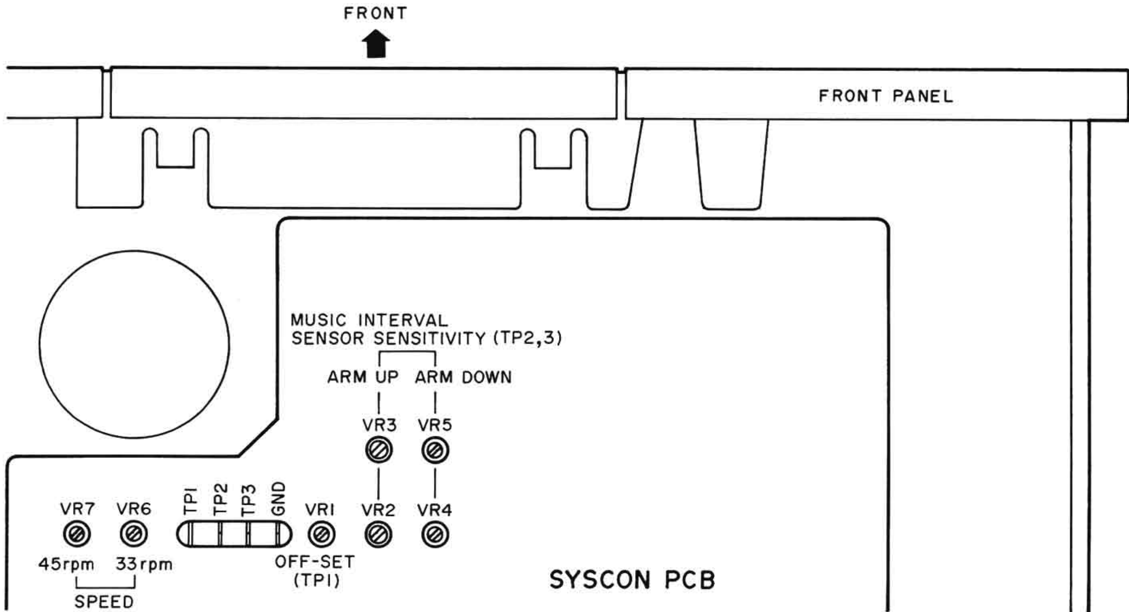
Fig. 6-5 Syscon PCB ADJ Points (Bottom View)
