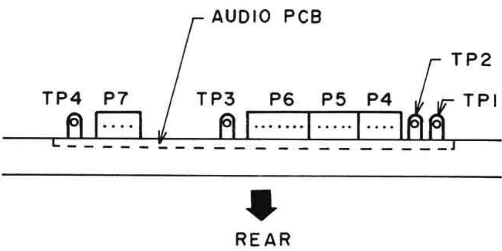
Fig. 6-3 Audio PCB Test Points (Top View)
