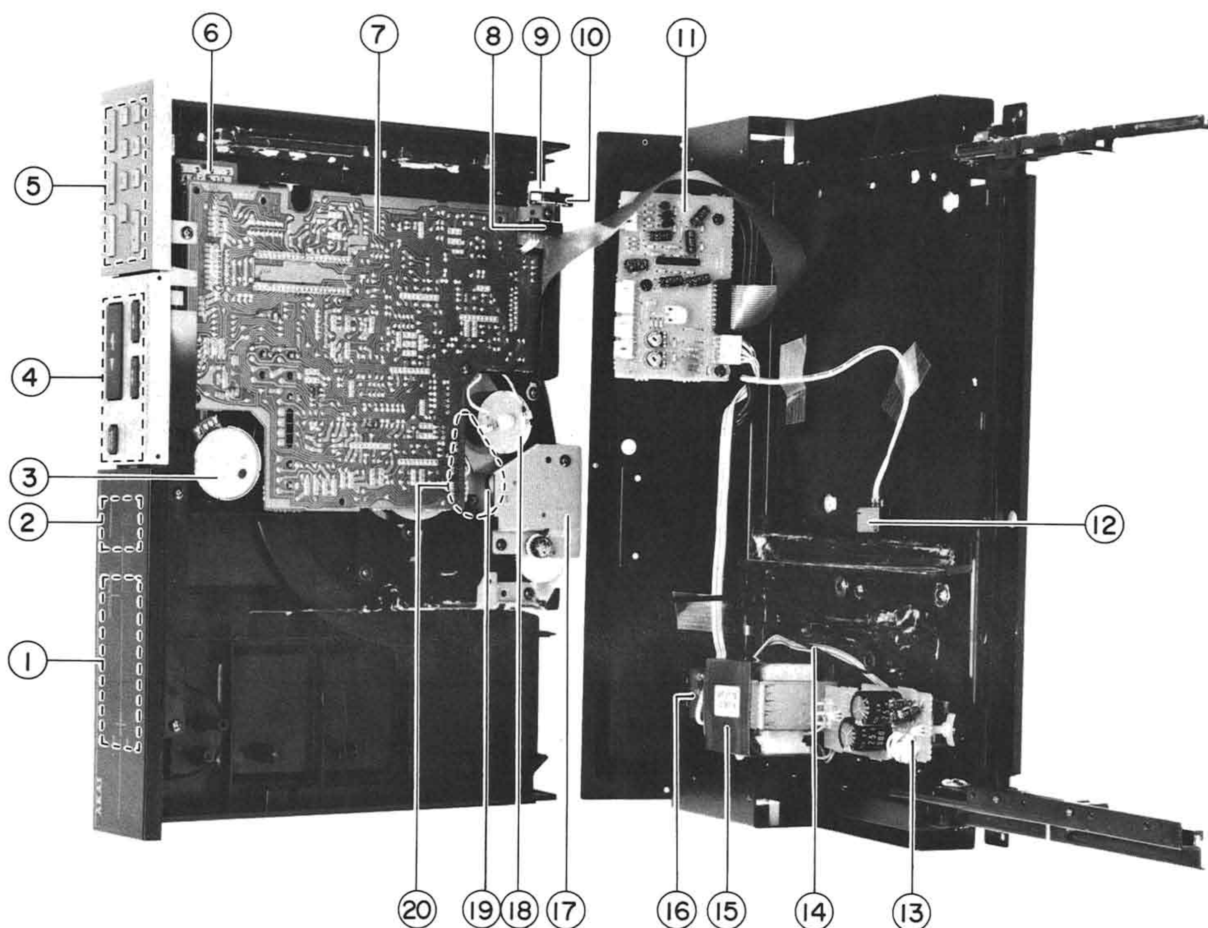
Fig. 4-2 Inside View
