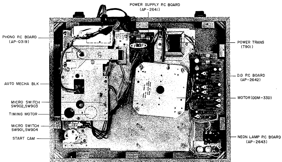
Fig. 3 Bottom View
