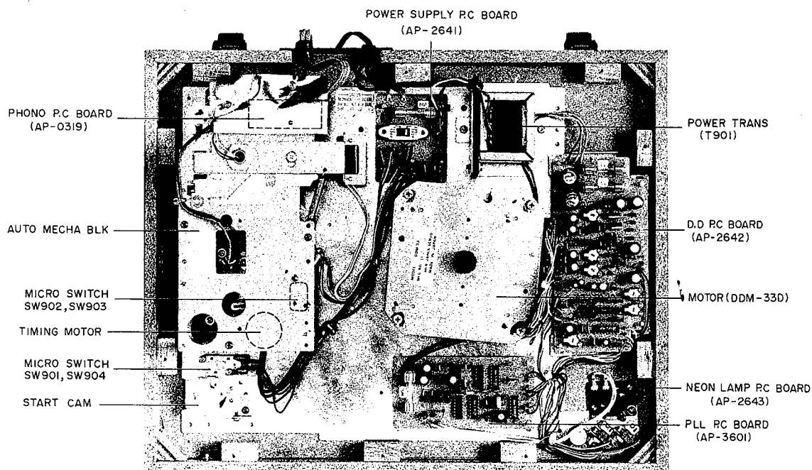
Fig. 4 Bottom View
