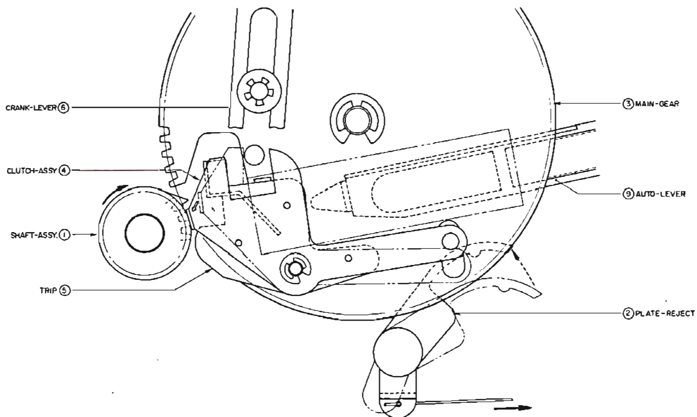
Fig. 13 FORCE CUT
