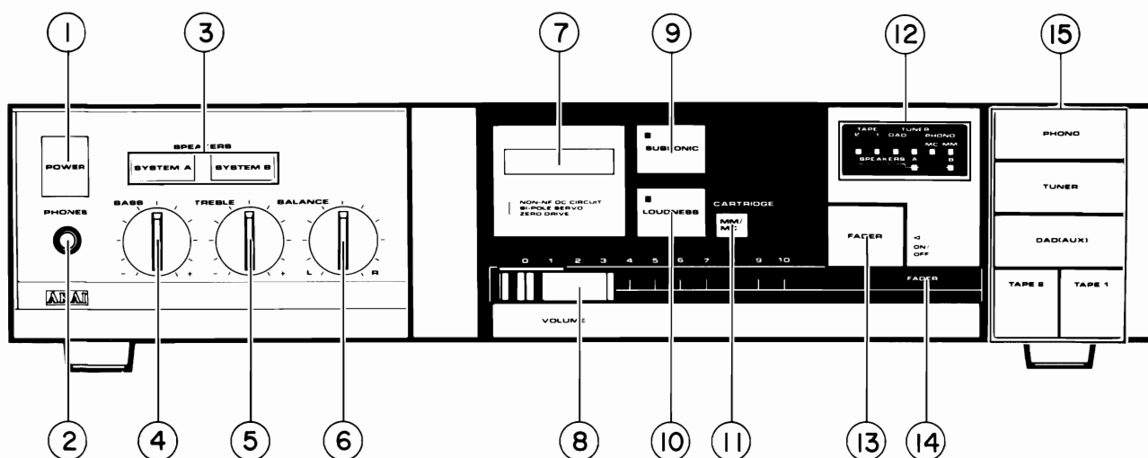
Fig. 3-1 Front View
