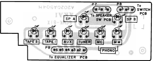
LED (C) PCB A2020A504H
