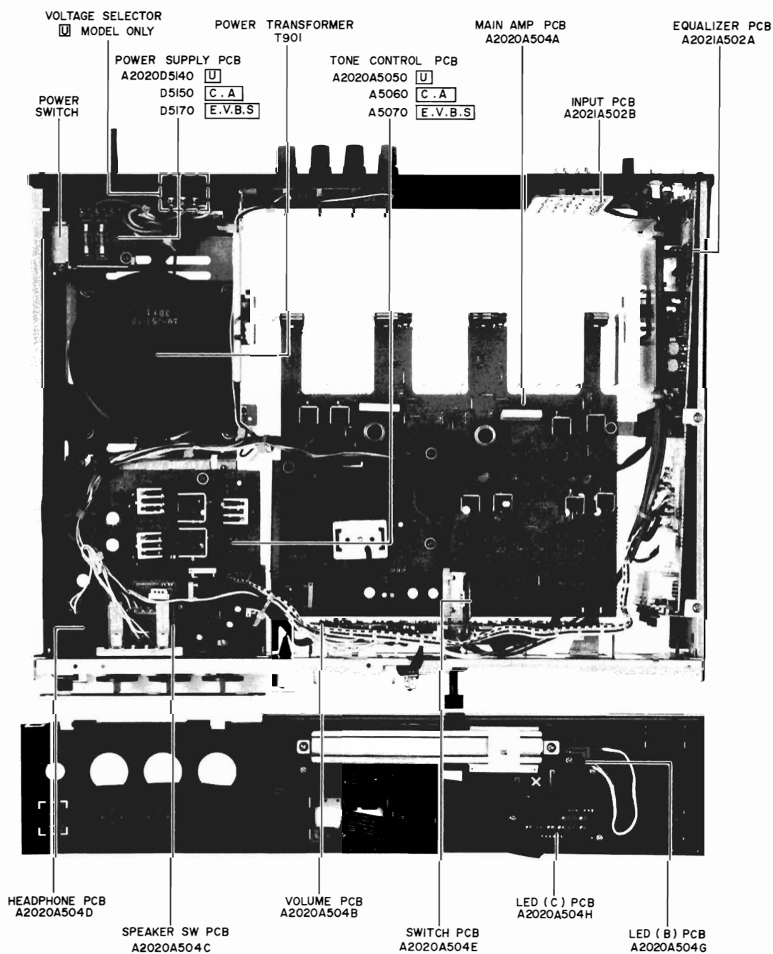
Fig. 4-2 Top View
