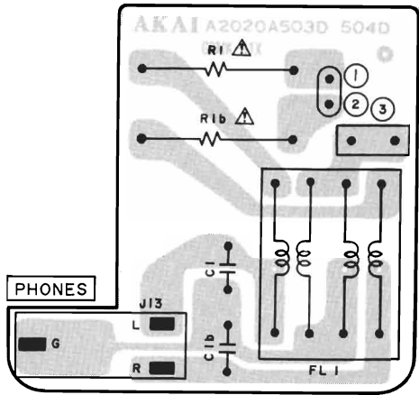
HEAD PHONE PCB A2020A504D V MODEL
