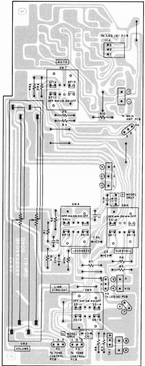
VOLUME PCB A2020A504B
