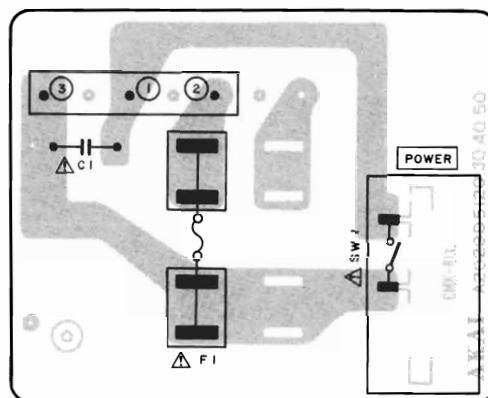
POWER SUPPLY PCB A2020D5150 [C, A]
