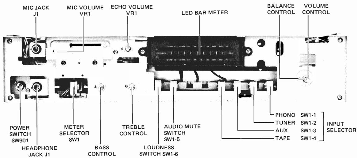
Fig. 2 Front View
