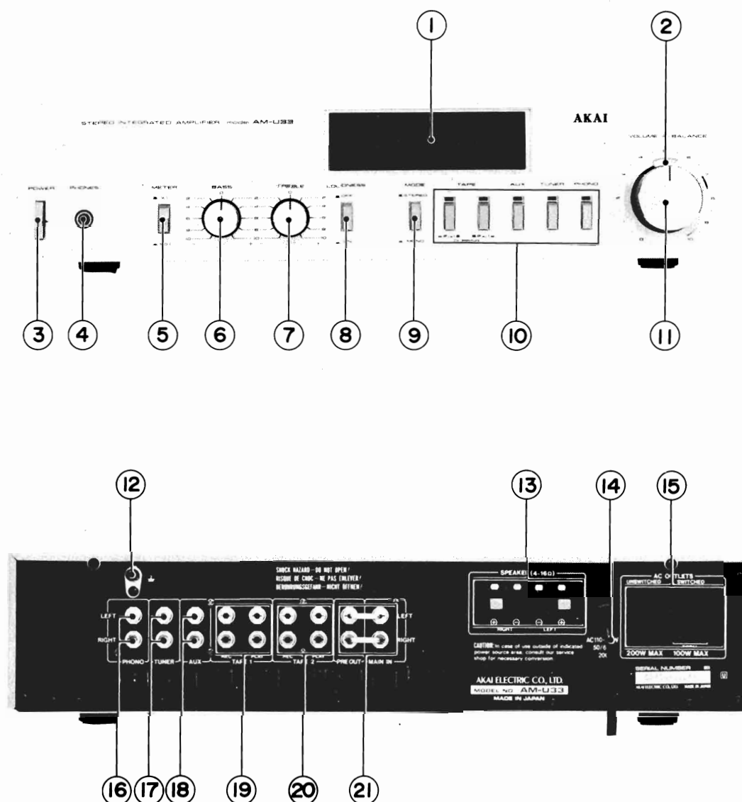
Fig. 1 Controls
