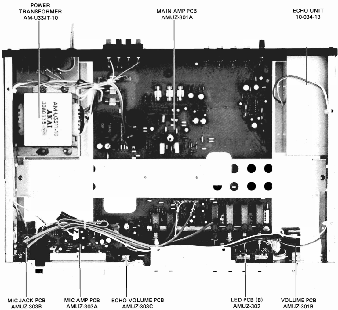
Fig. 3 Top View
