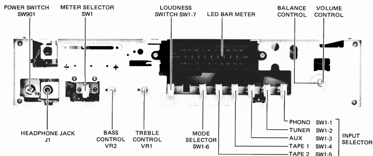
Fig. 2 Front View
