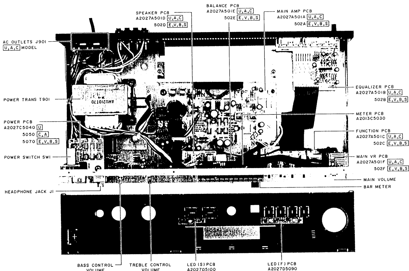
Fig. 4 Top View
