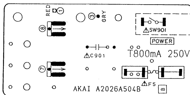
POWER SW PCB A2026A504B B
