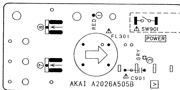
POWER SW PCB A2026A505B V
