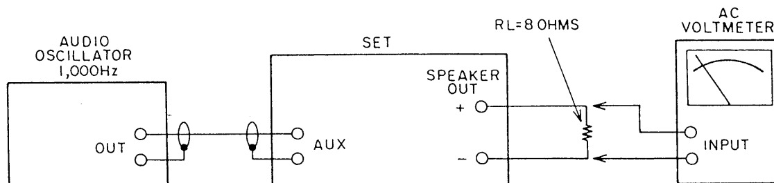
Fig. 5 Instrument Connections
