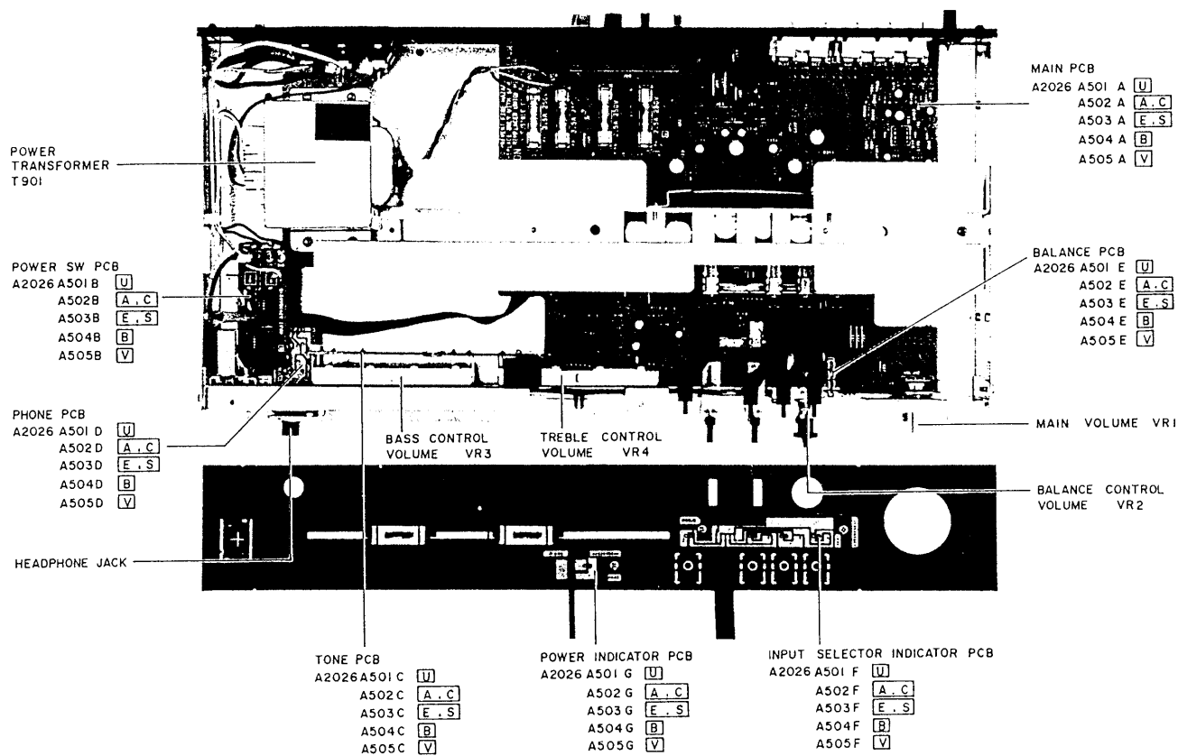
Fig. 4 Top View
