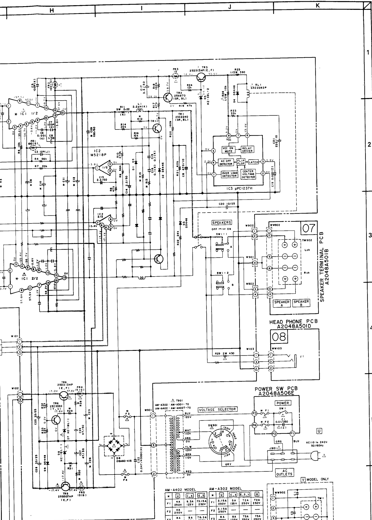
MAIN PCB A2048A501A
