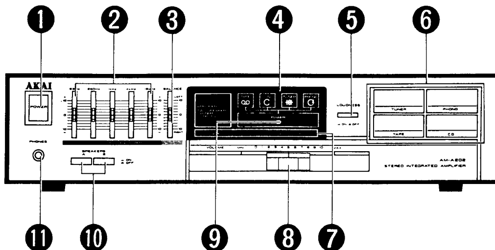
Fig. 3-1 Controls for Models AM-A102, AM-A202
