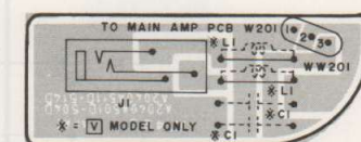
HEADPHONE PCB A2040A50ID [U] 502D [C.A] 503D [E.B.S] 504D [V]
