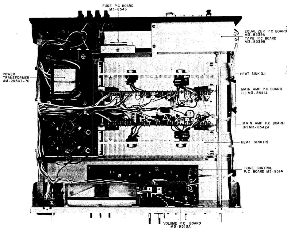
Fig. 3 Top View
