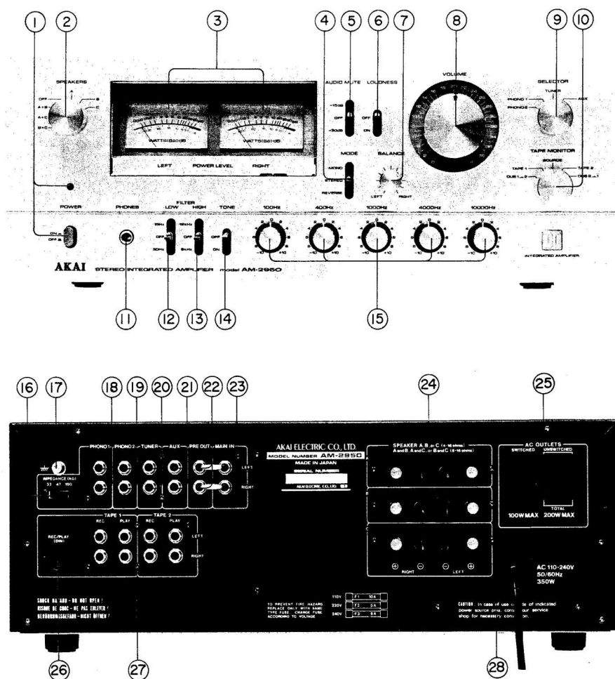
Fig. 1 Controls
