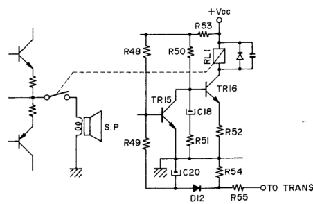
Fig. 8 Mute Circuit
