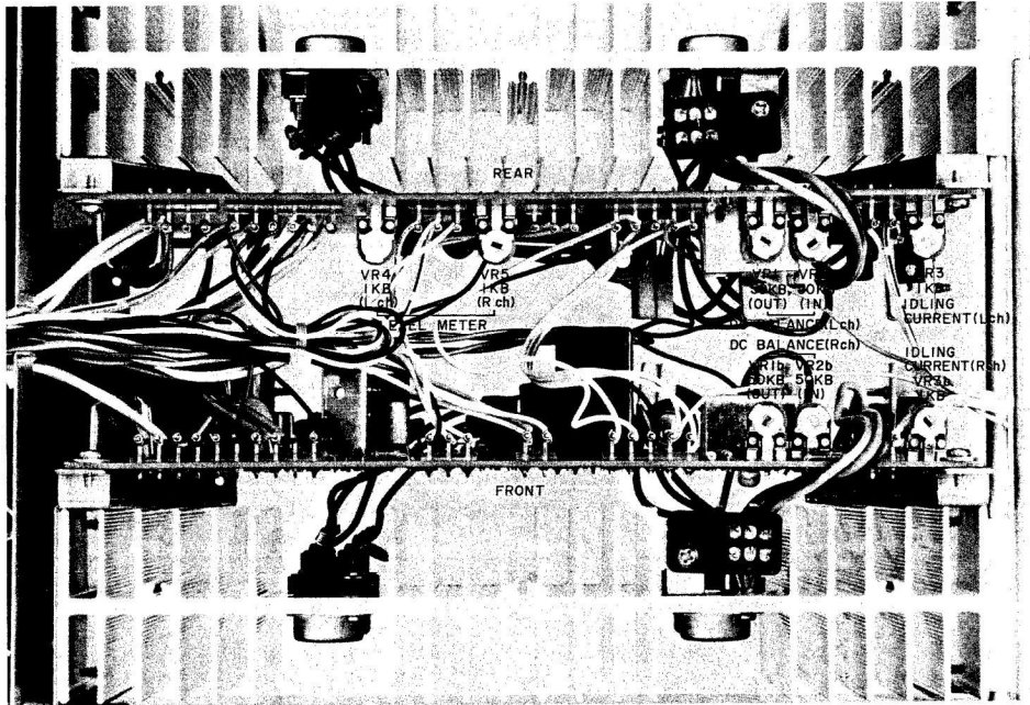
Fig. 14 Main Amp Adjust Point
