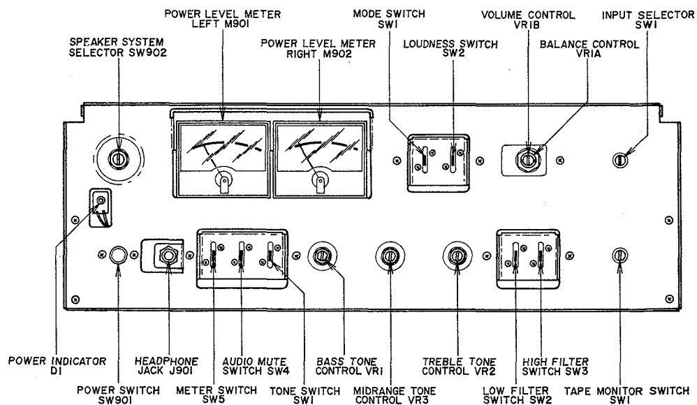
Fig. 3 Front View
