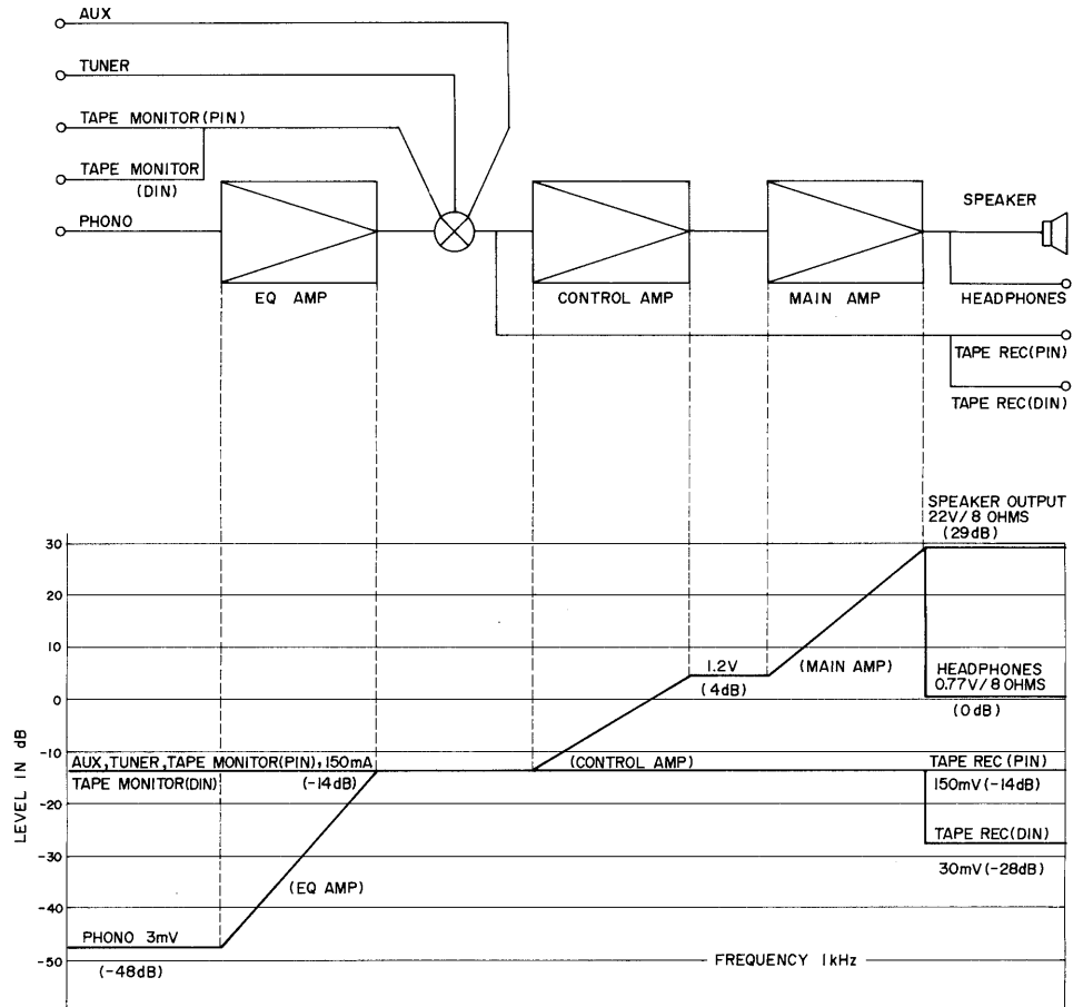
Fig. 4 Level Diagram of Model AM-2600
