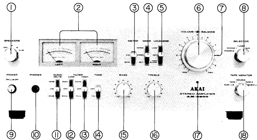
Fig. 1 Controls
