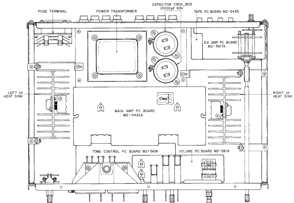
Fig. 2 Top View
