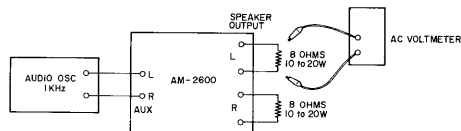
Fig. 6 Level Meter Adjustment
