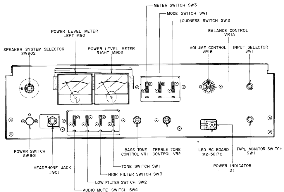
Fig. 3 Front View
