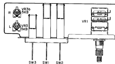
Fig. 7 Volume P.C Board M2-5619
