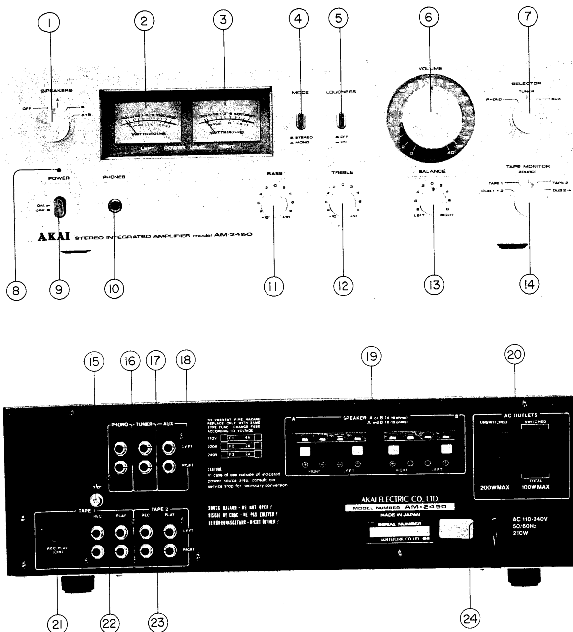
Fig. 2 Controls AM-2450
