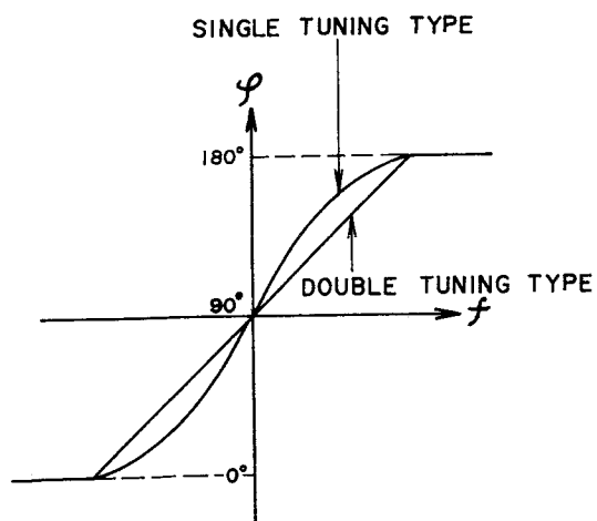
Fig. 10 Tuning Curve
