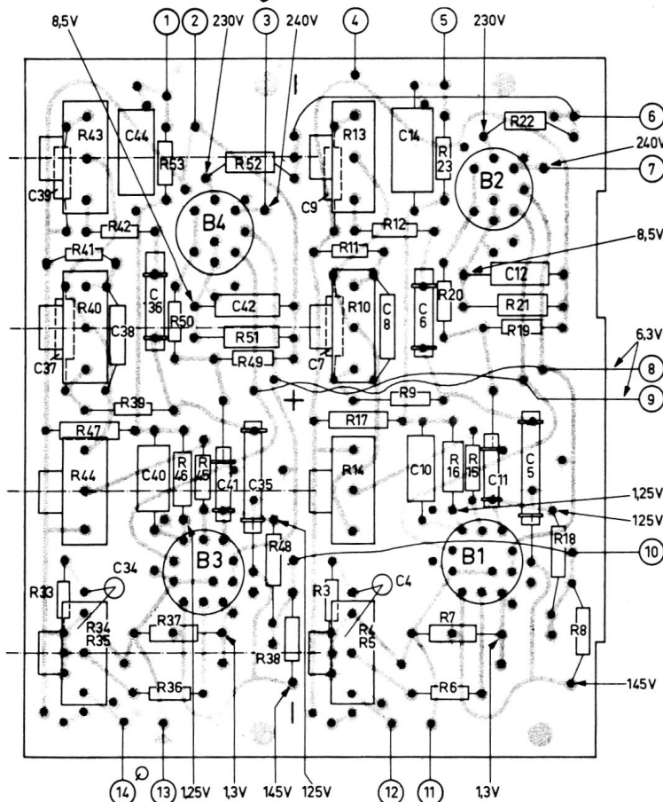
Circuit Board Layout
