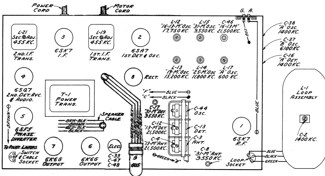
Fig. 1—Chassis Layout and Alignment Adjustments
