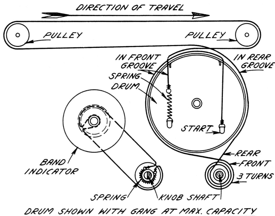
Fig. 5—Drive Cords
