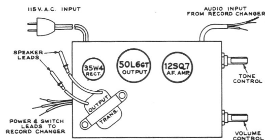
Amplifier Top View
