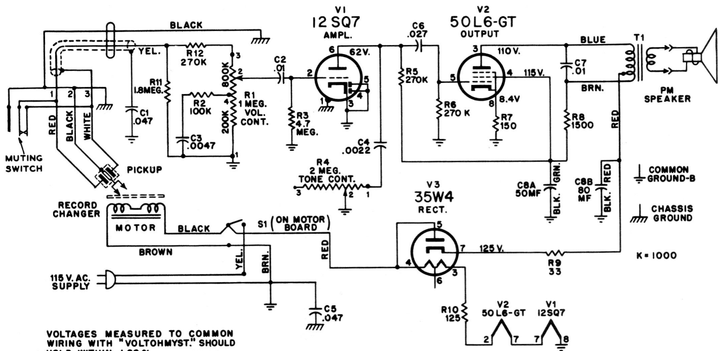
Schematic Diagram
