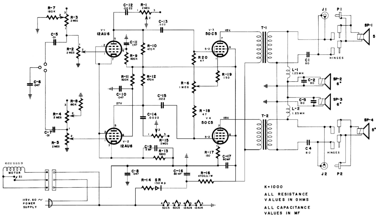
SCHEMATIC DIAGRAM
