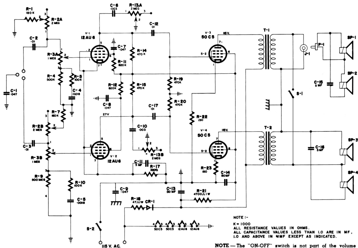
SCHEMATIC DIAGRAM
