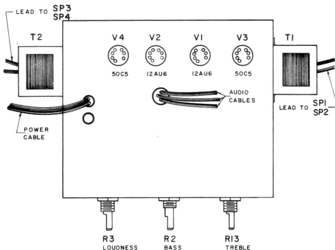
Chassis Layout — Top View
