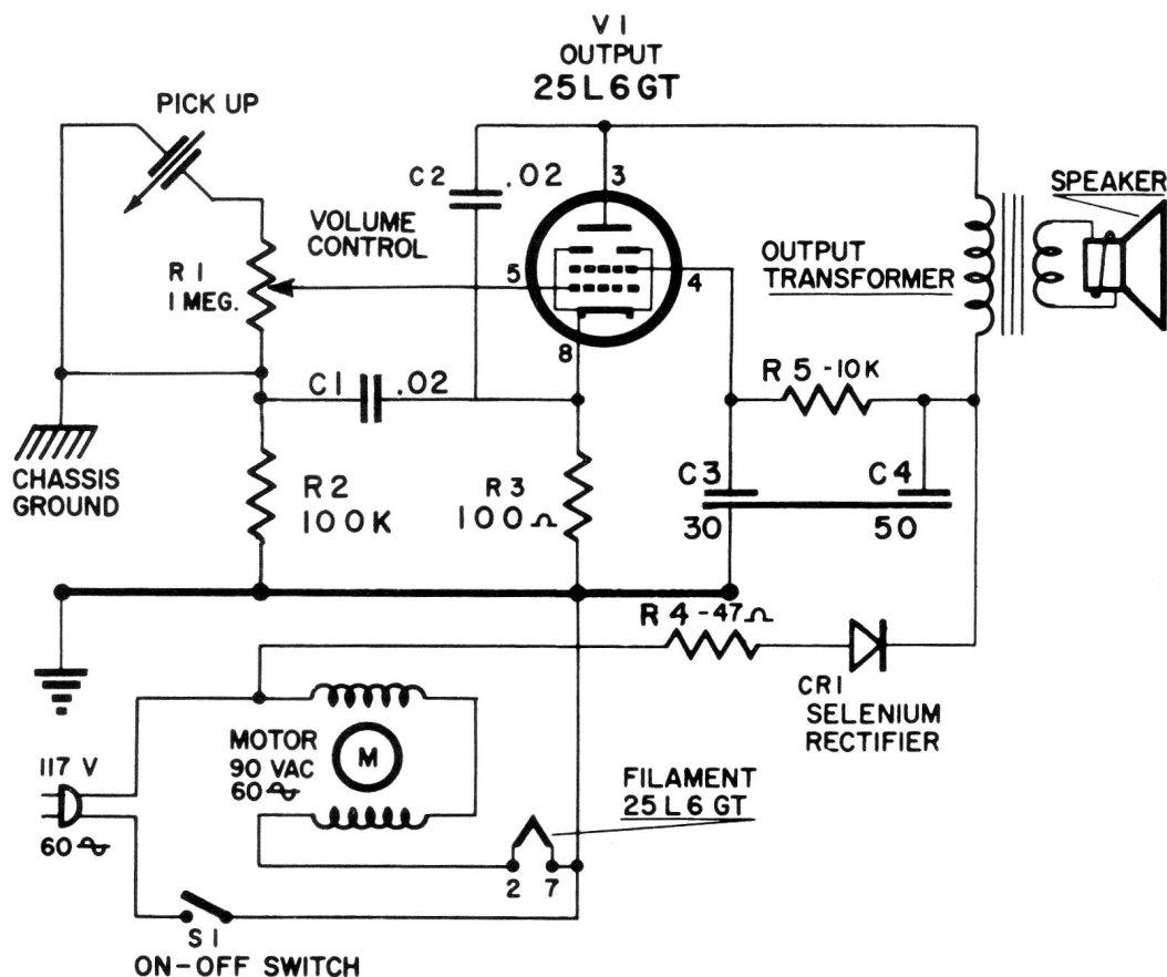
SCHEMATIC DIAGRAM FOR MODEL K-571
