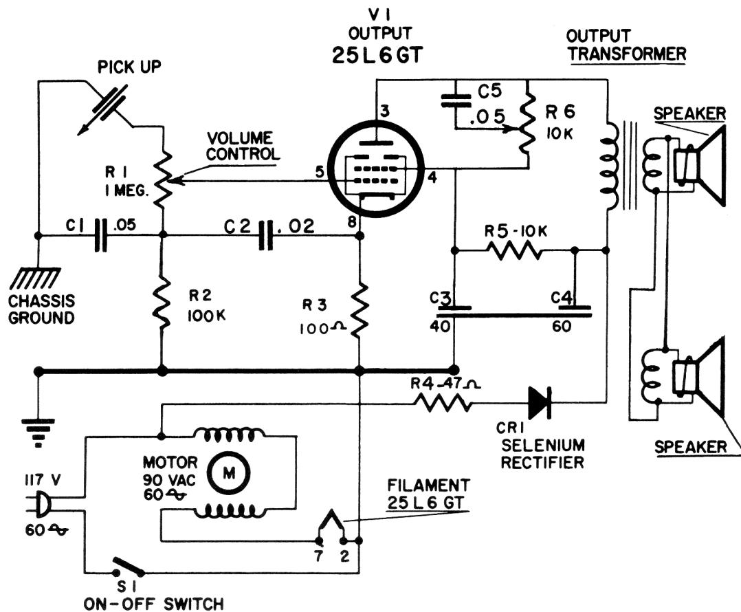
SCHEMATIC DIAGRAM FOR MODEL K-573
