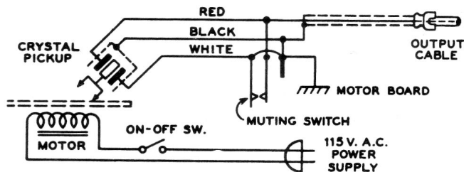
Schematic Diagram for Model K-181
