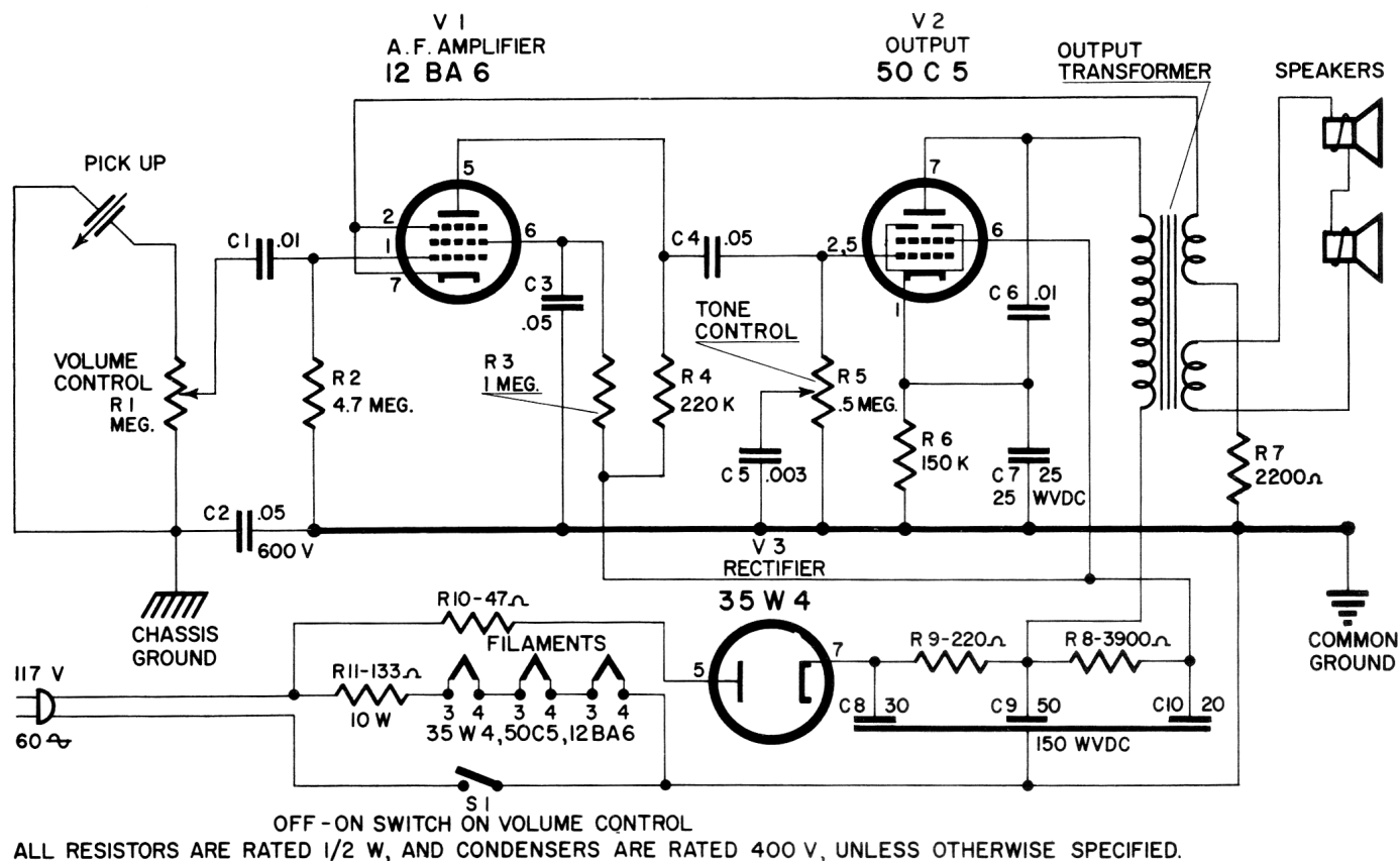
Schematic Diagram for Models F-180, F-182
