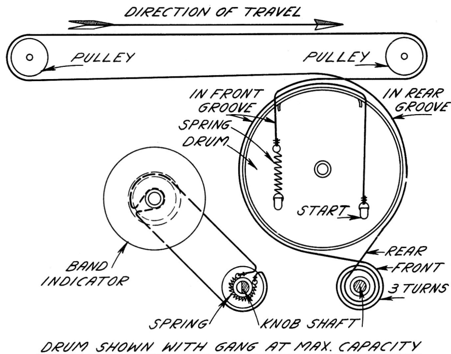
Fig. 5—Drive Cords
