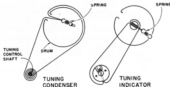
Diagram of Drive Cord with Condenser Rotor Closed (Extreme Counter-clockwise Position)
