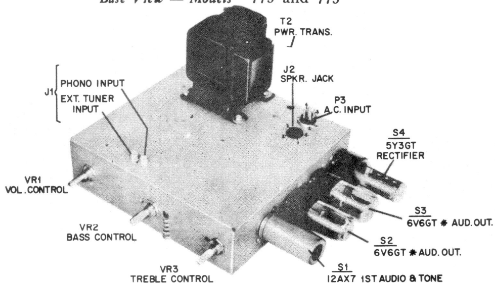
Base View — Models 773 and 775
