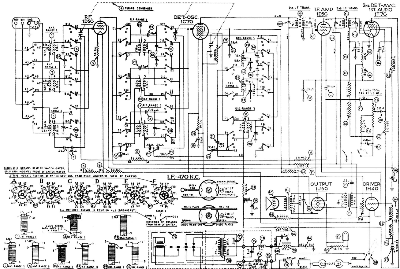
Fig. 5—Schematic Diagram
