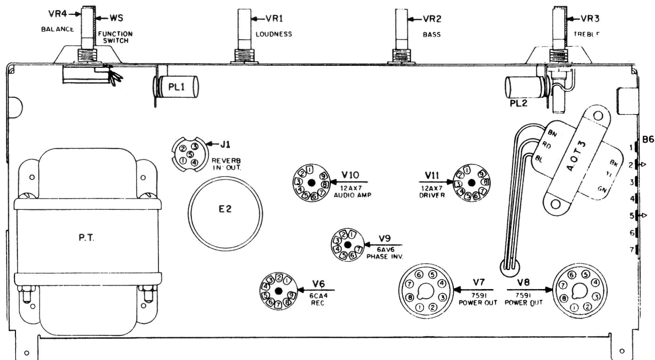
Figure 18. Bottom View, 1748-1750 Amplifier Chassis Showing Component Location
