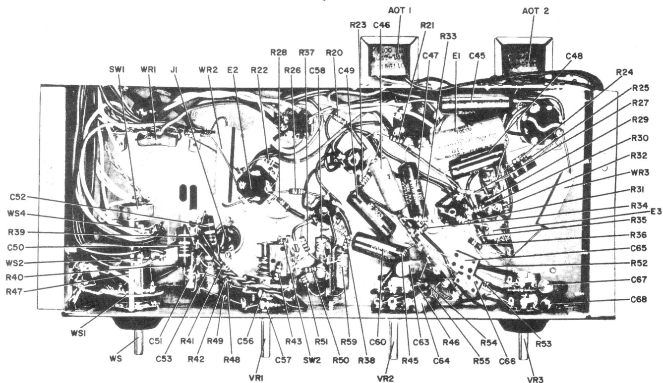
Figure 16. Bottom View , 1748-1750 Amplifier Chassis
