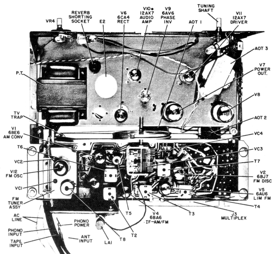
Figure 15. Top View , 1748-1750 Chassis Tuner
