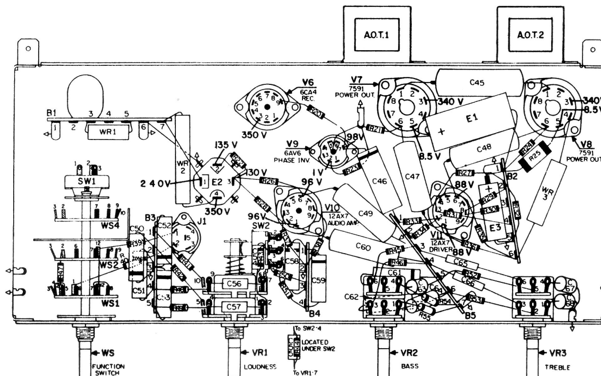
Figure 18. Bottom View, 1748-1750 Amplifier Chassis Showing Component Location
