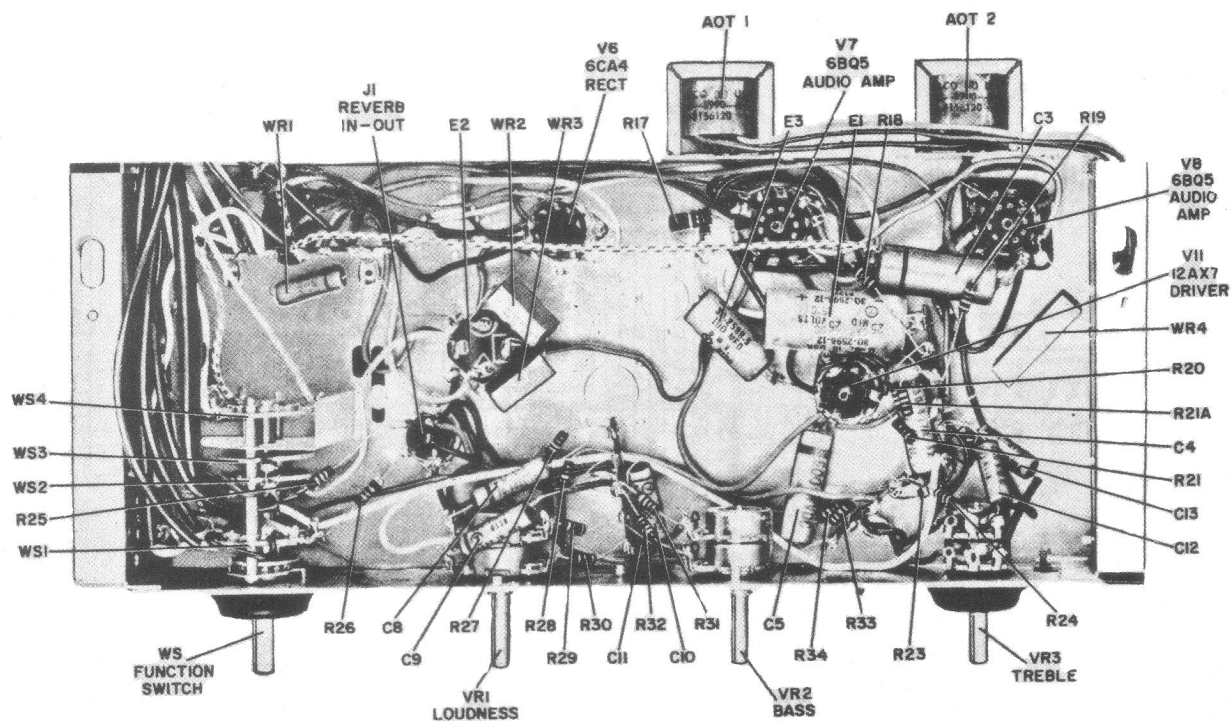
Figure 11. Bottom View, 1742 Amplifier Chassis
