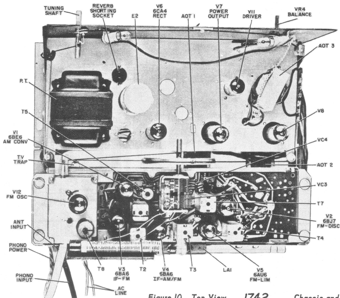
Figure 10. Top View, 1742 Chassis and Tuner
