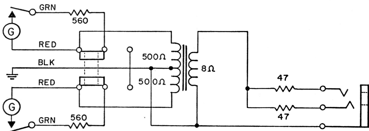
EARLIER HAMMOND ORGAN MODELS WITH PREAMP. ONLY
