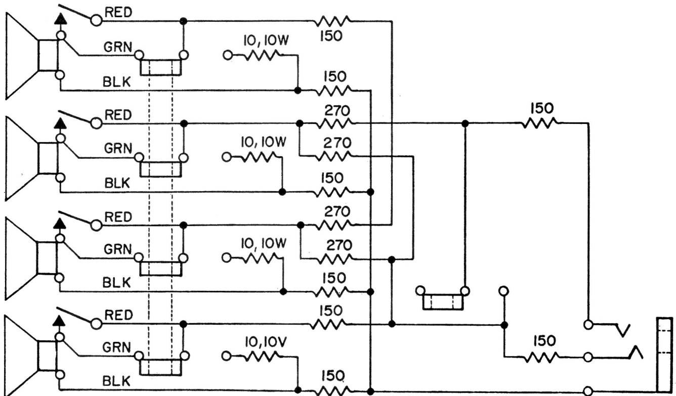
ORGANS WITH FOUR AMPLIFIER SYSTEMS
