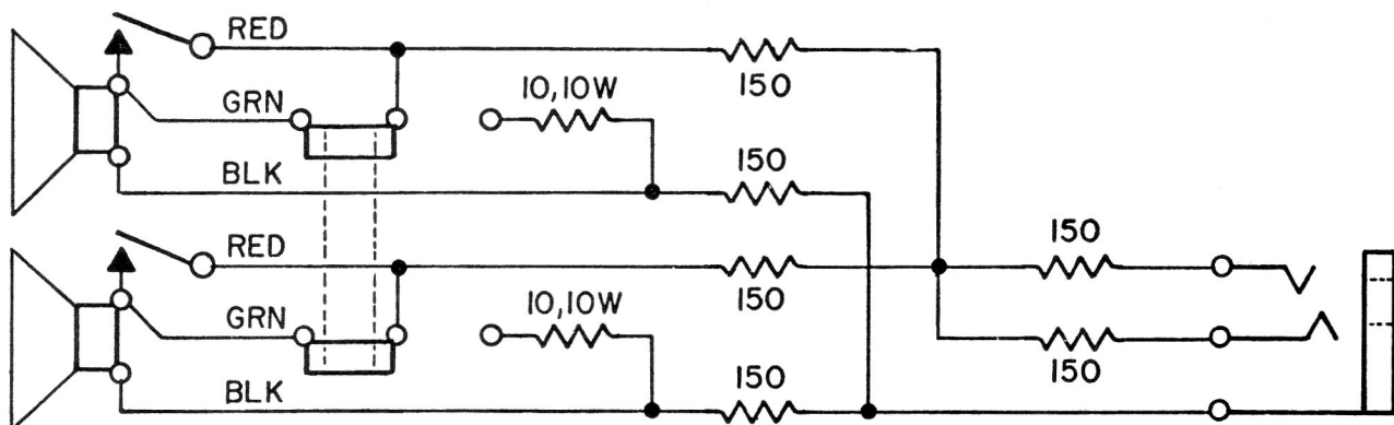
ORGANS WITH AN EXTRA AMPLIFIER FOR REVERB, E.T.C.
