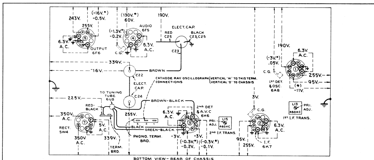
Figure 1—Radiotron Socket Voltages and Trimmer Locations
