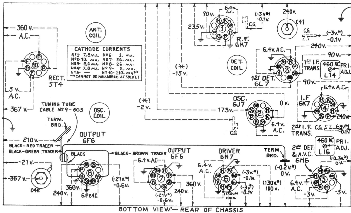
Figure 2—Radiotron Socket Voltages, Coil, and Trimmer Locations
