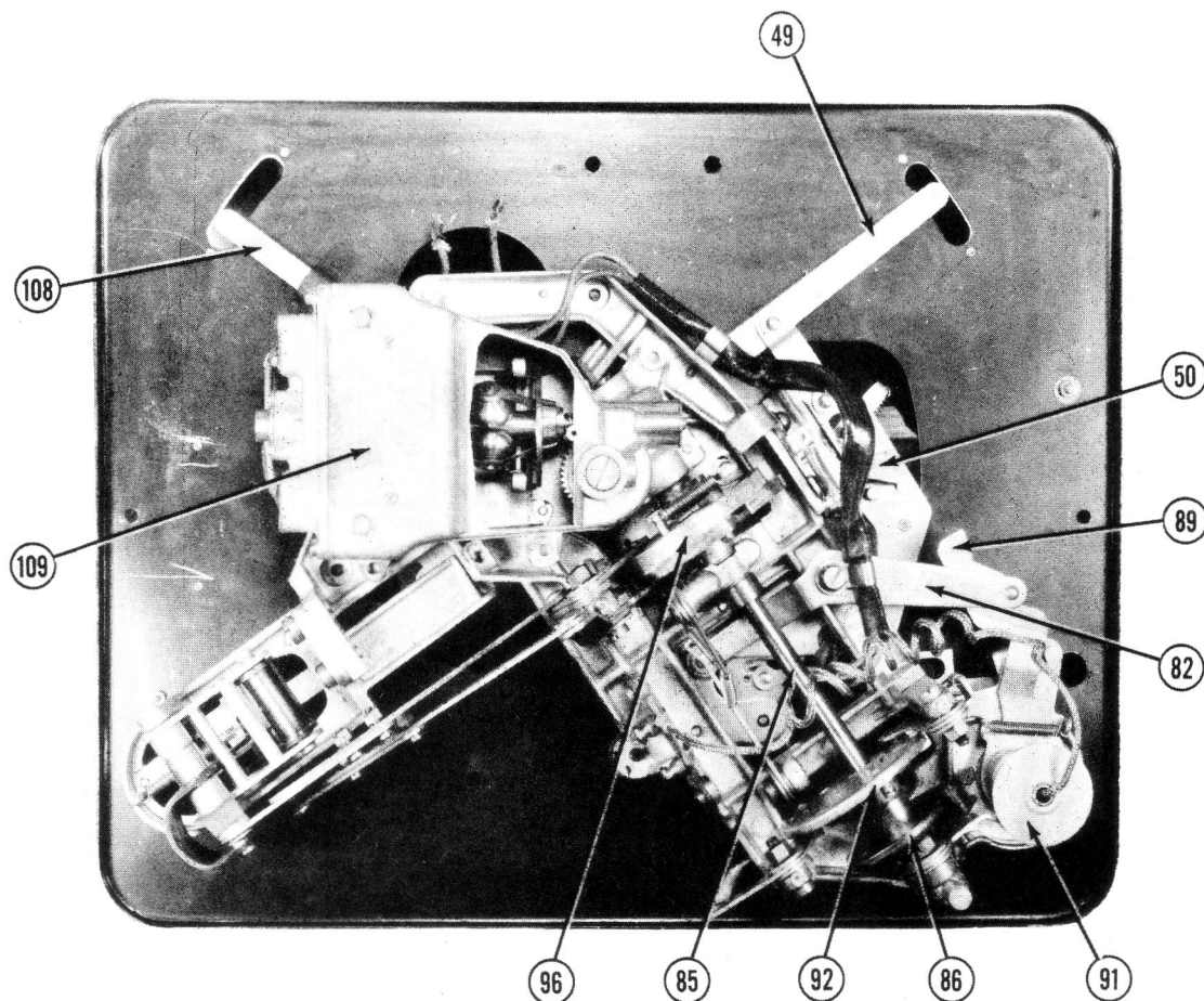
FIG. 7—BOTTOM VIEW
