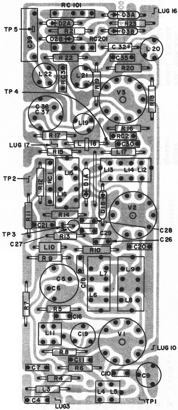
COMPONENT VIEW
