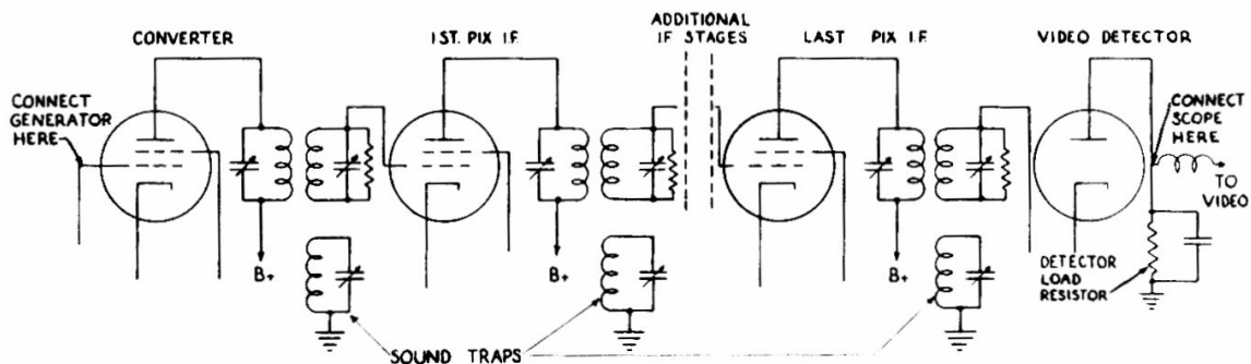
TYPICAL TELEVISION INTERMEDIATE FREQUENCY AMPLIFIER AND DETECTOR
