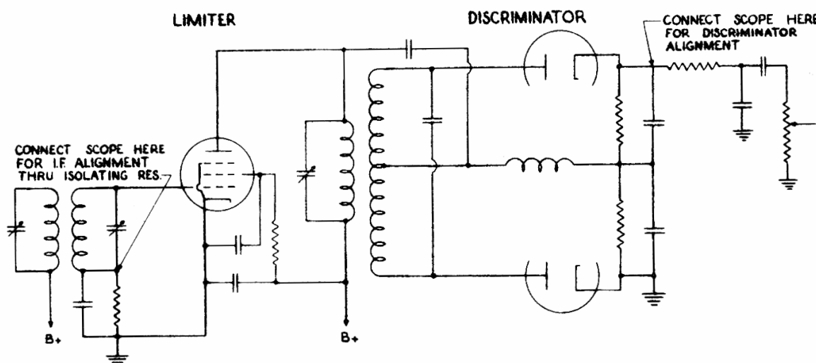
FOSTER - SEELEY DISCRIMINATOR
