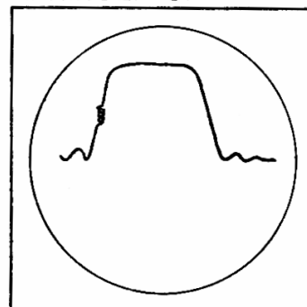
VIDEO IF RESPONSE CURVE WITH MARKER ON SLOPE
