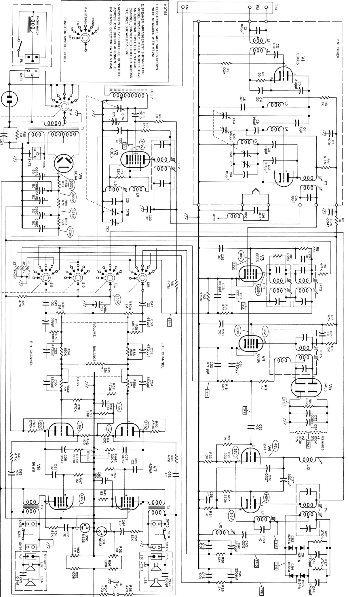
CLAIRTONE CHASSIS C303 used in MODELS S253, S303, S373, S383, S393
