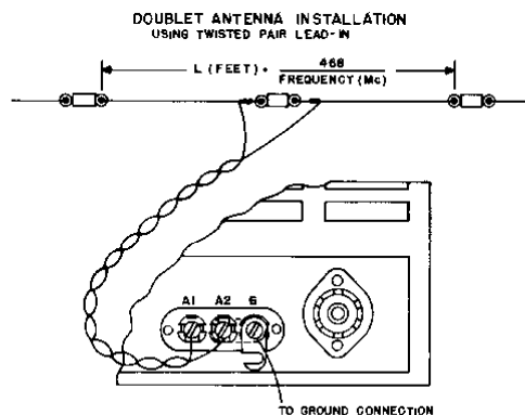
FIG. 3 DOUBLET ANTENNA INSTALLATION
