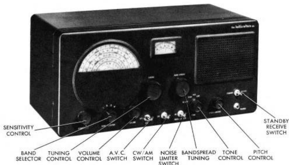
FIG. 1 MODELS S-40B & S-40BU
