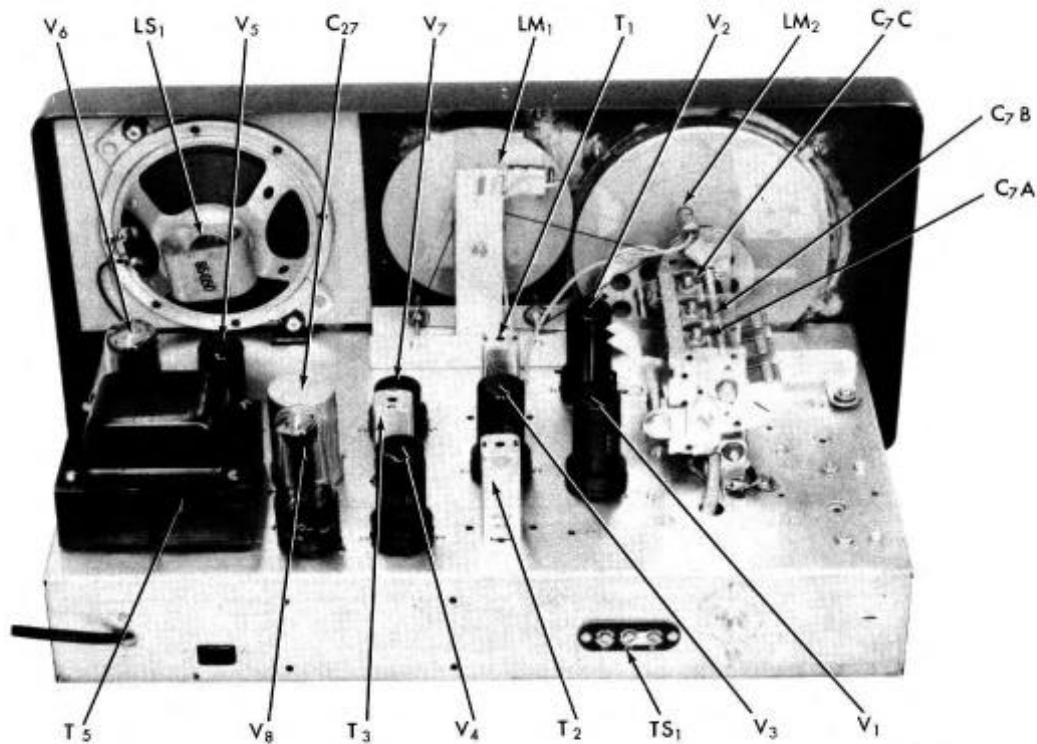
FIG. 8 TOP VIEW - COMPONENT LOCATION
