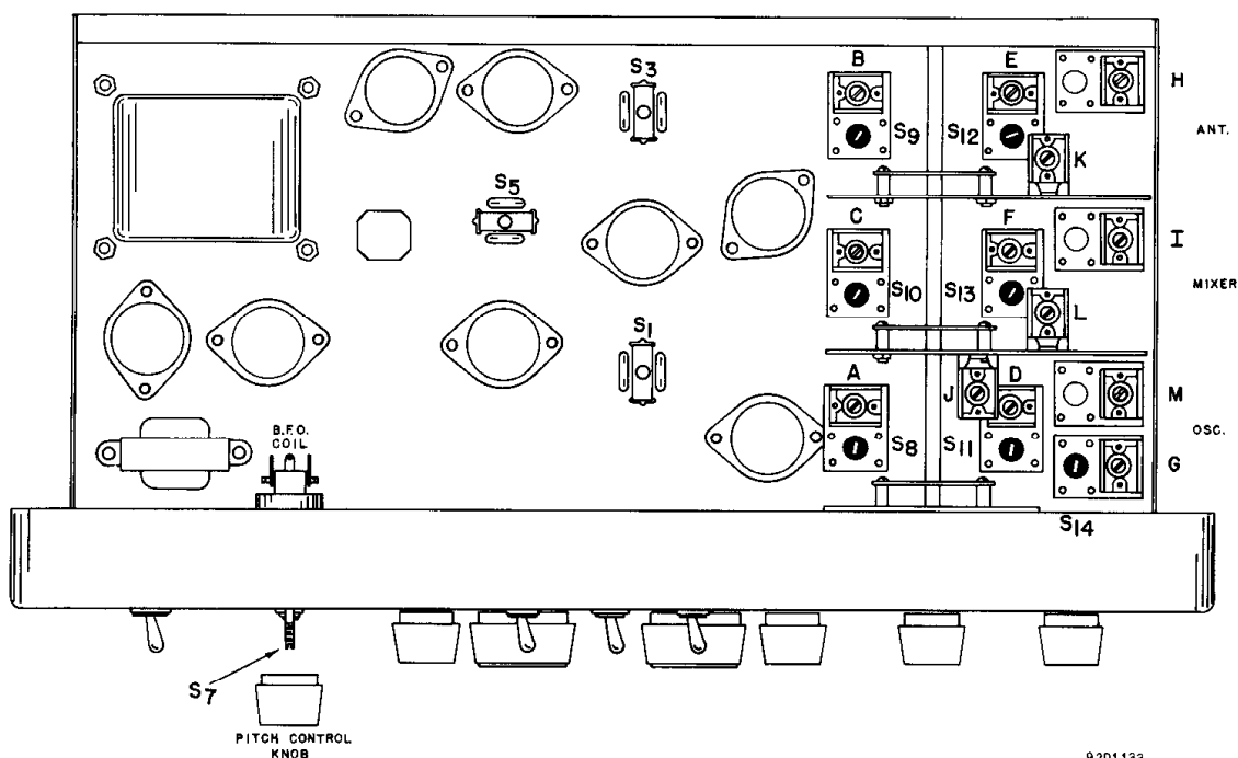
FIG. 6 BOTTOM VIEW - LOCATION OF ALIGNMENT ADJUSTMENTS
