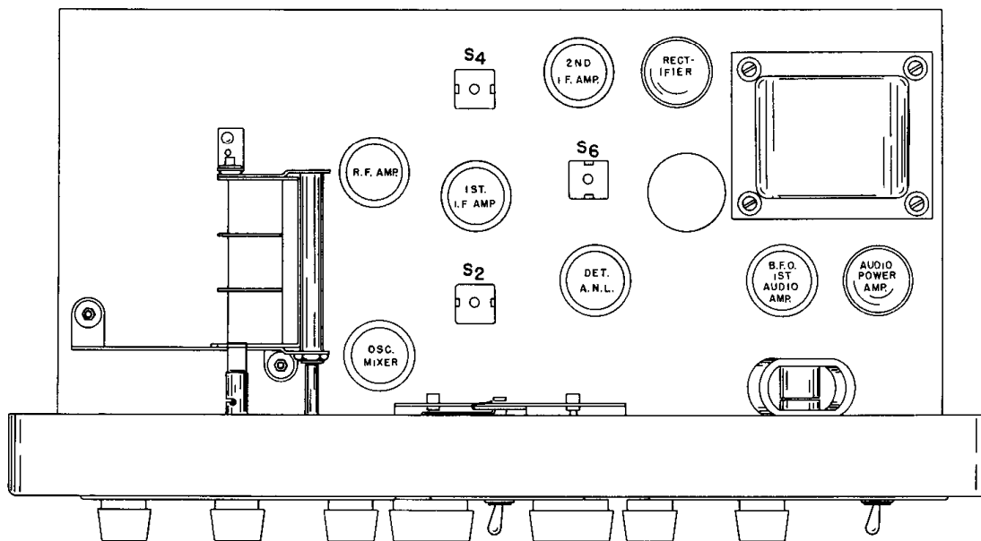
FIG. 5 TOP VIEW - LOCATION OF ALIGNMENT ADJUSTMENTS
