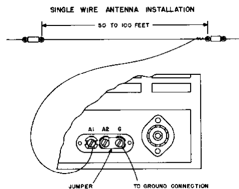
FIG. 2 SINGLE WIRE ANTENNA INSTALLATION
